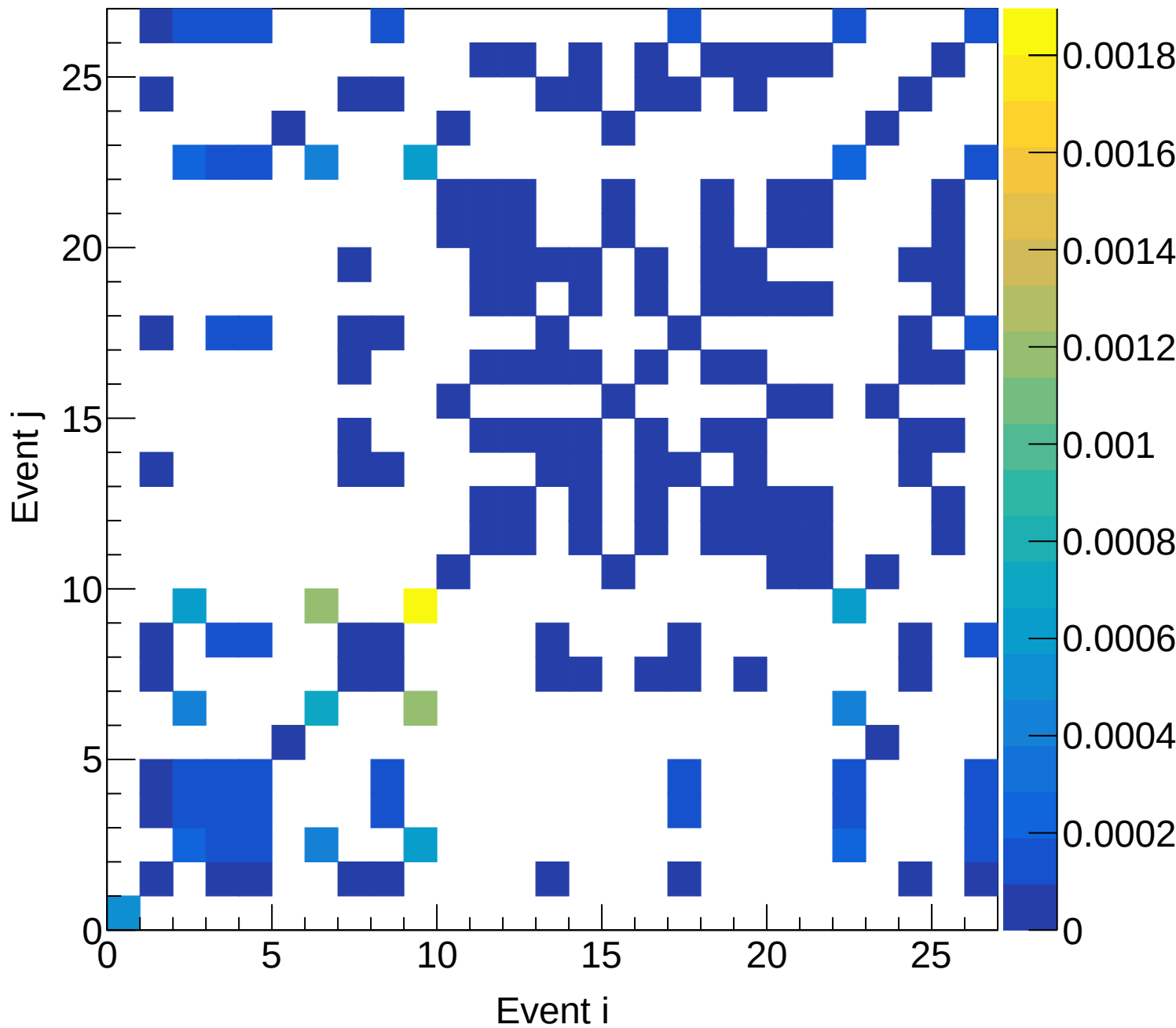
LH2 (total) Covariance | M: [6.0, 6.3) xF: [0.00, 0.05)
