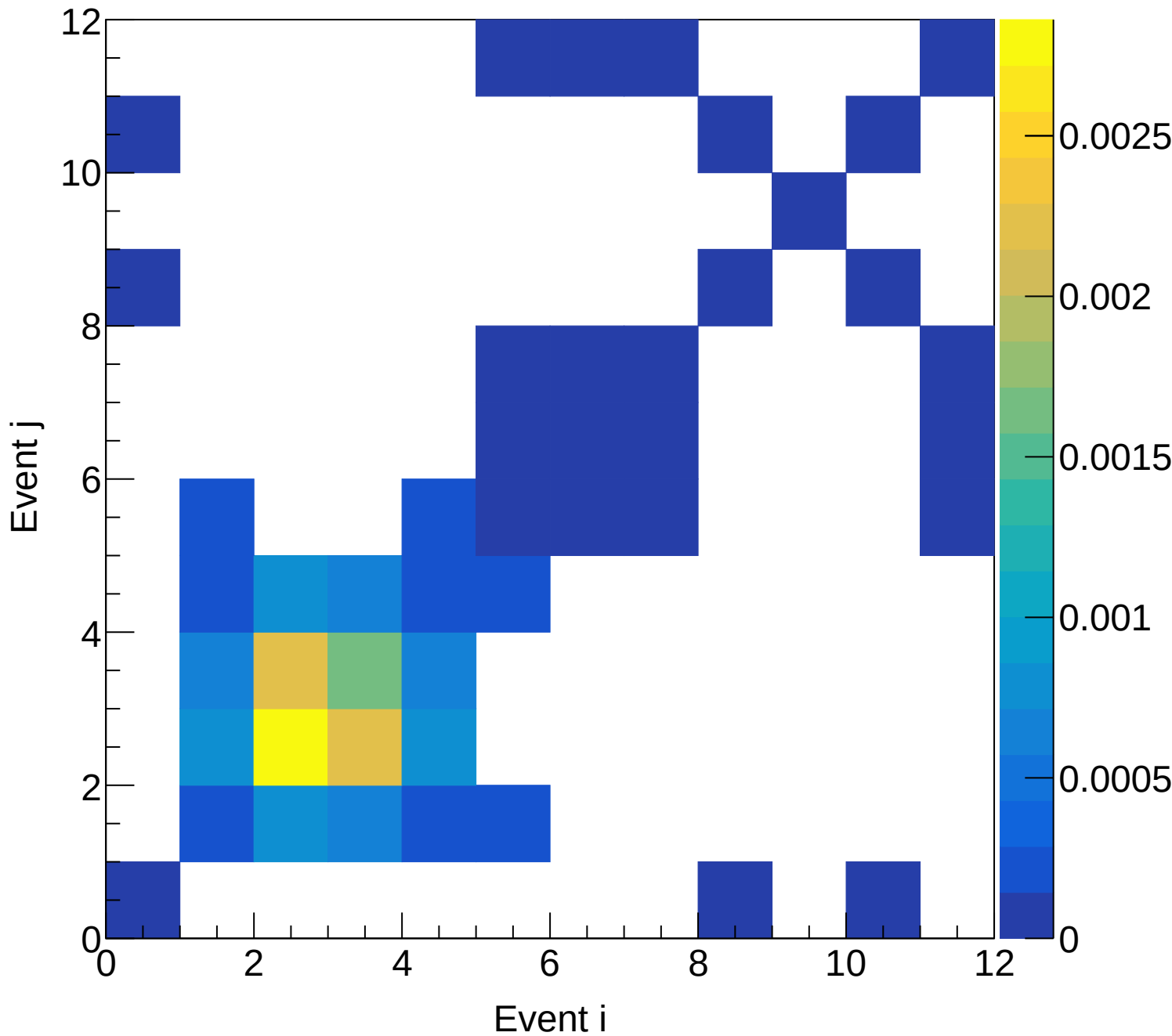
LH2 (total) Covariance | M: [6.6, 6.9] xF: [0.00, 0.05]
