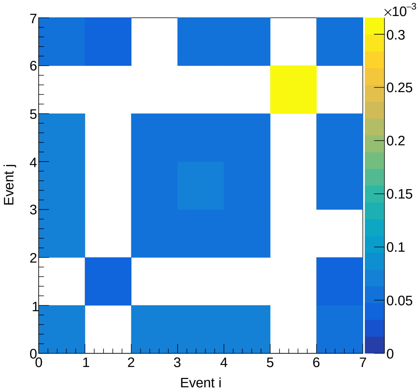
LH2 (total) Covariance | M: [6.9, 7.5) xF: [0.05, 0.10)
