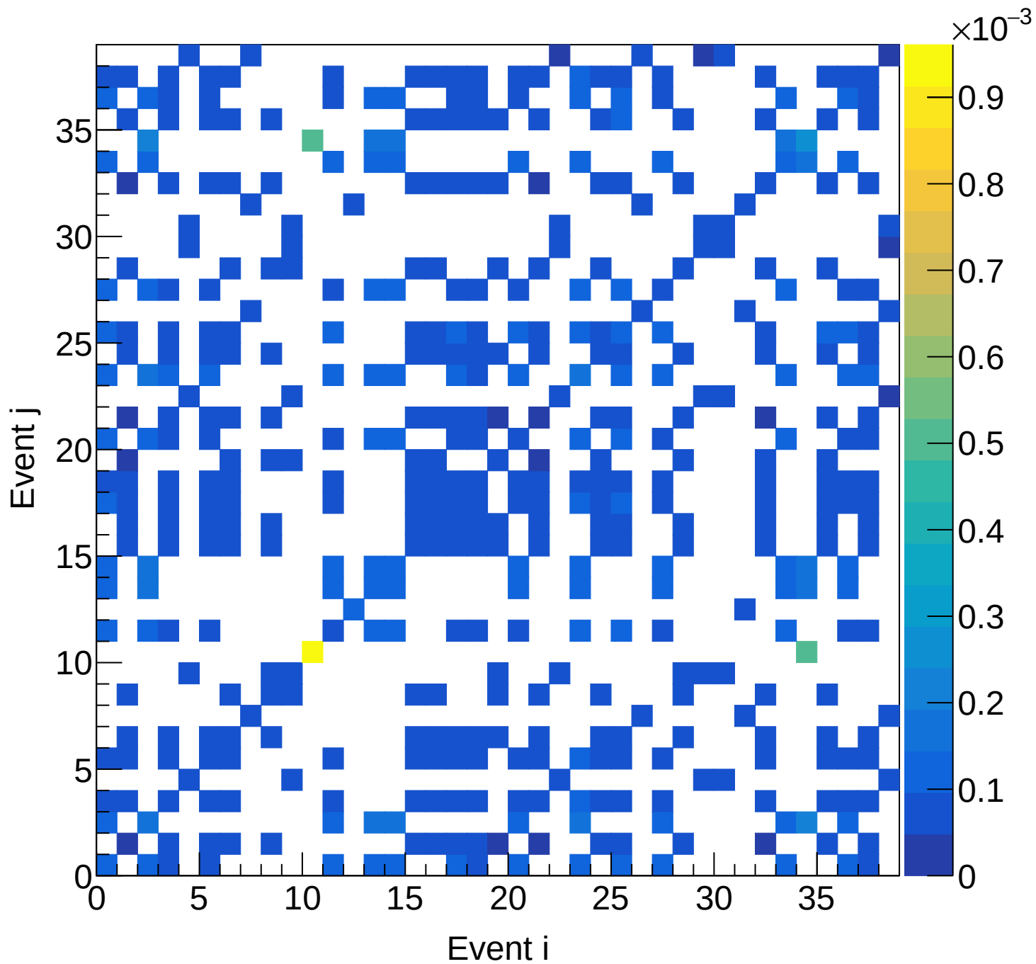
LH2 (total) Covariance | M: [4.5, 4.8) xF: [0.05, 0.10)
