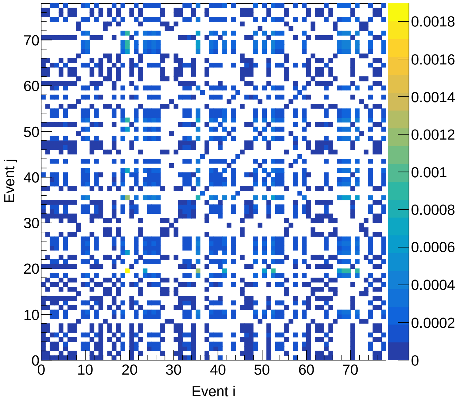
LH2 (total) Covariance | M: [5.4, 5.7) xF: [0.05, 0.10)
