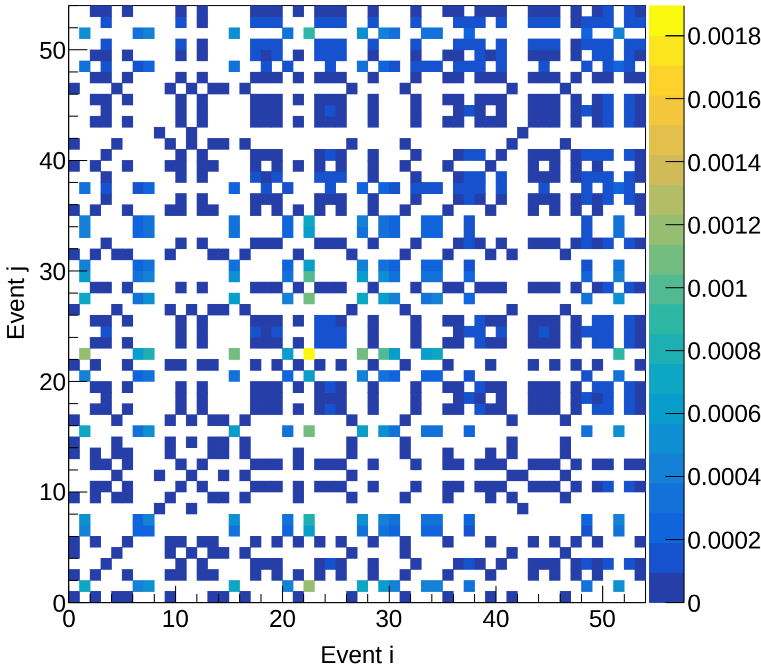
LH2 (total) Covariance | M: [5.7, 6.0] xF: [0.05, 0.10]
