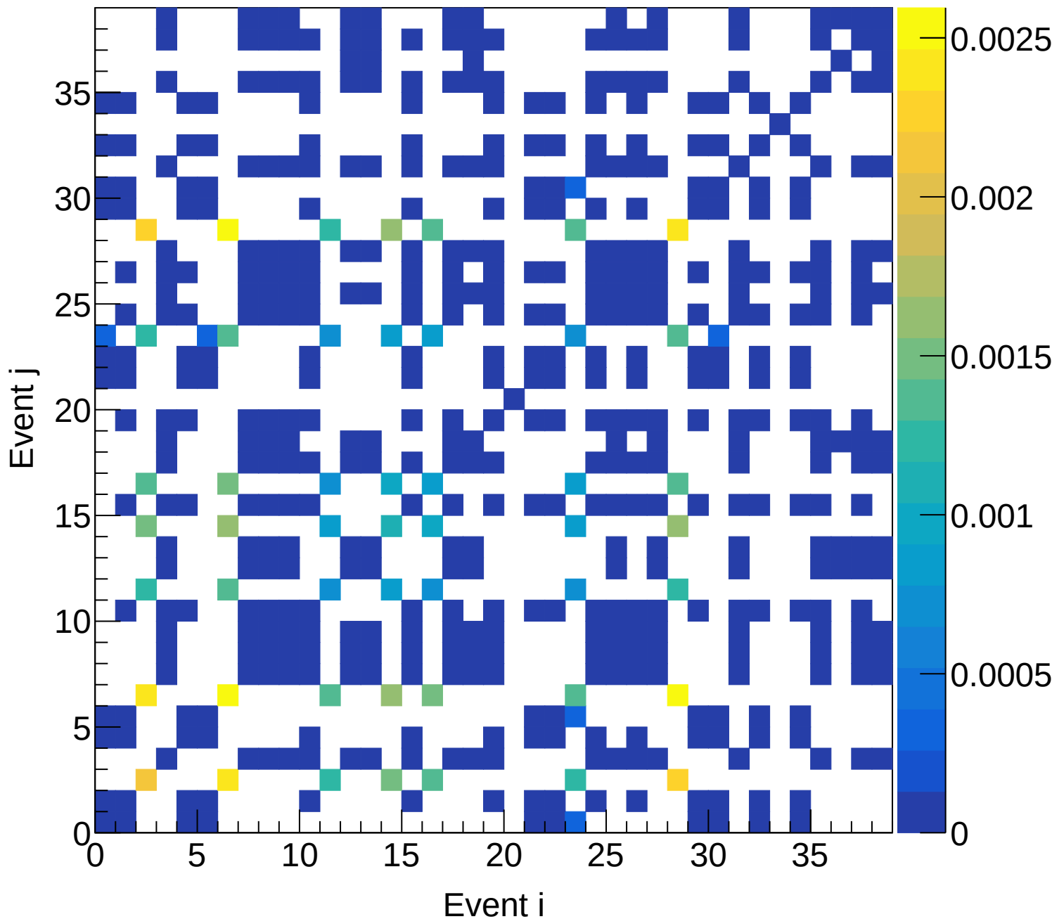
LH2 (total) Covariance | M: [6.0, 6.3] xF: [0.05, 0.10]
