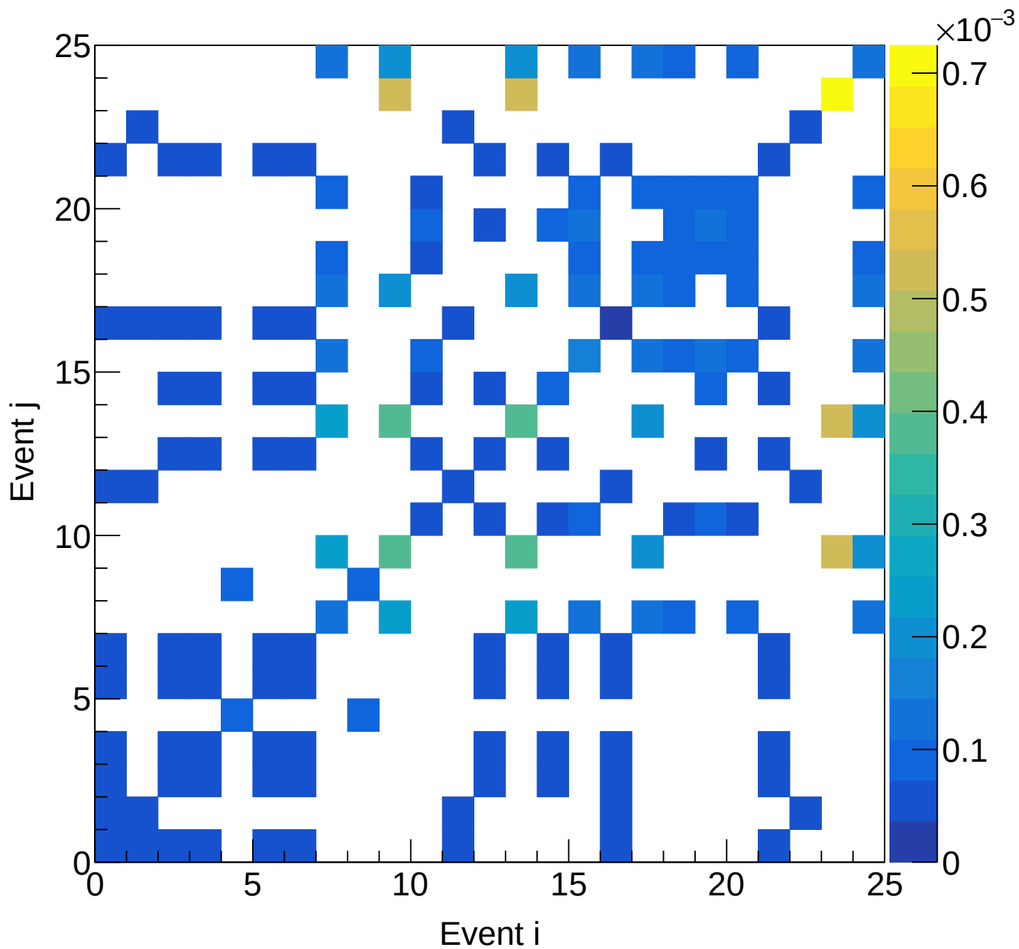
LH2 (total) Covariance | M: [6.3, 6.6] xF: [0.05, 0.10)
