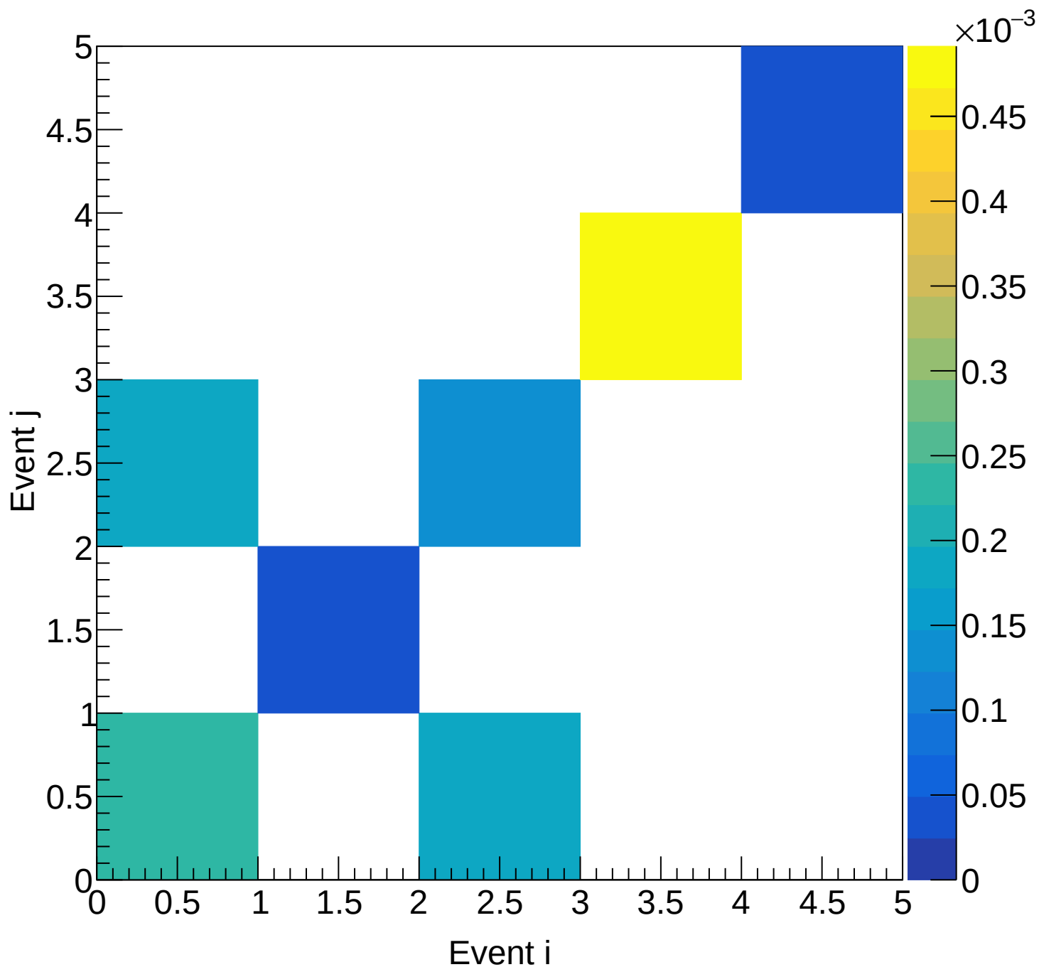
LH2 (total) Covariance | M: [6.6, 6.9) xF: [0.05, 0.10)
