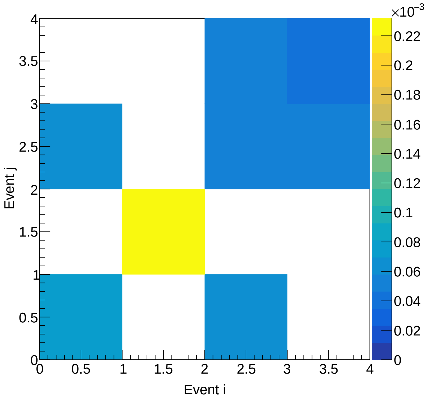
LH2 (total) Covariance | M: [3.9, 4.2) xF: [0.10, 0.15)
