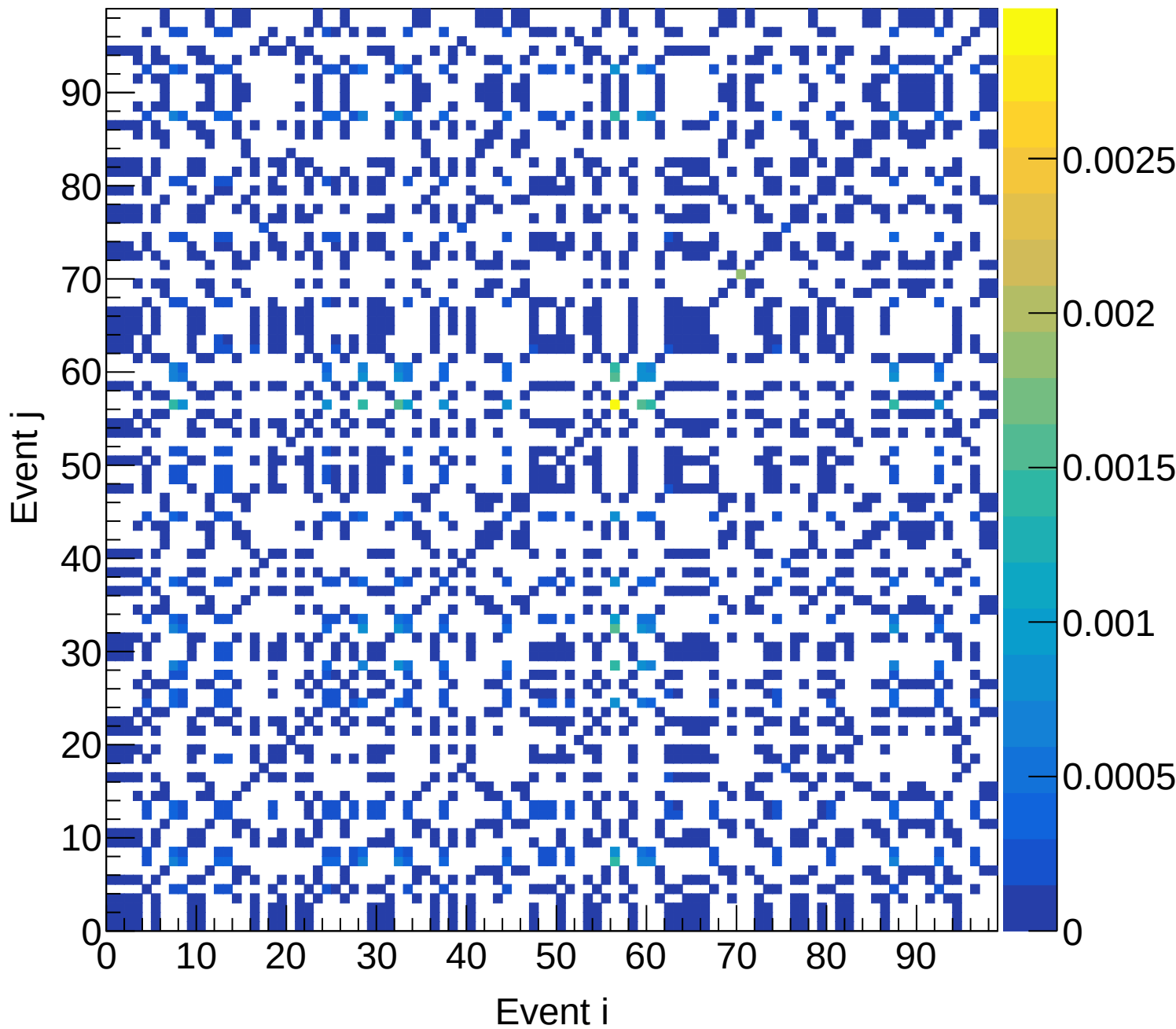
LH2 (total) Covariance | M: [4.5, 4.8) xF: [0.10, 0.15)
