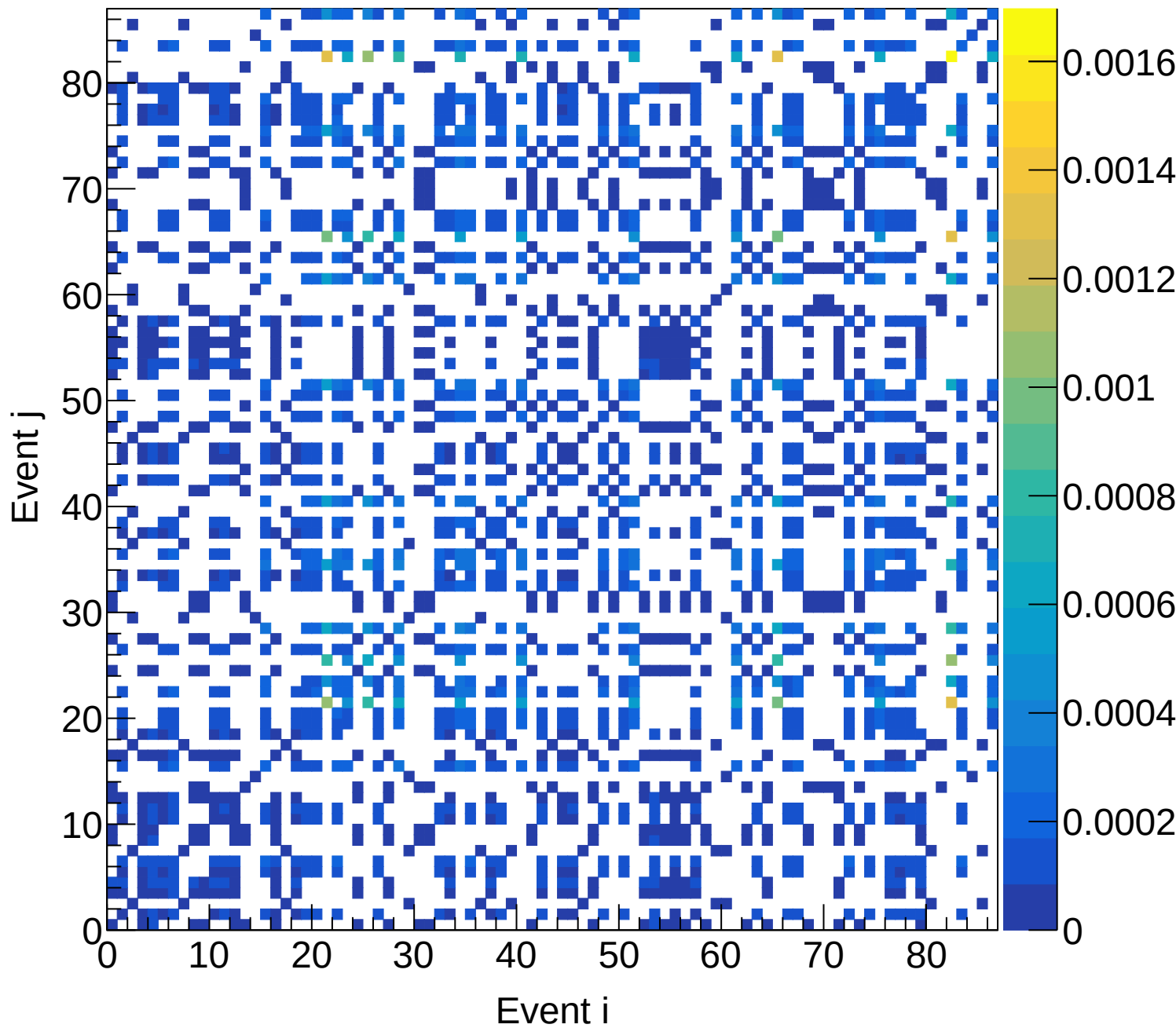
LH2 (total) Covariance | M: [5.4, 5.7] xF: [0.10, 0.15]
