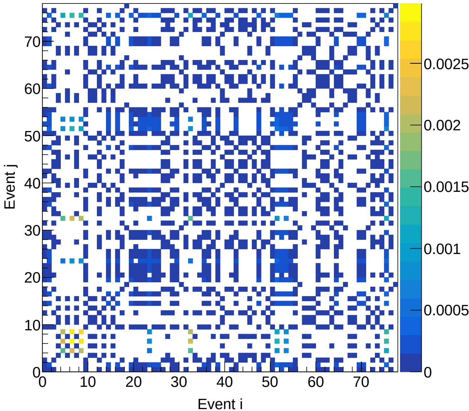
LH2 (total) Covariance | M: [5.7, 6.0) xF: [0.10, 0.15)
