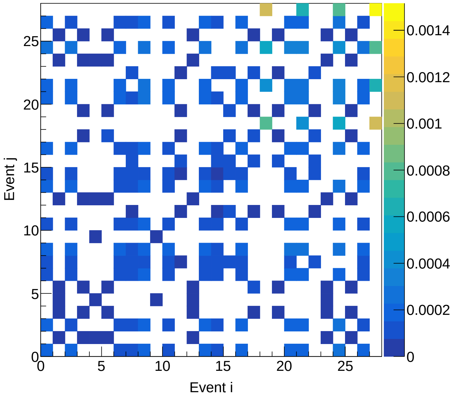
LH2 (total) Covariance | M: [6.3, 6.6) xF: [0.10, 0.15)
