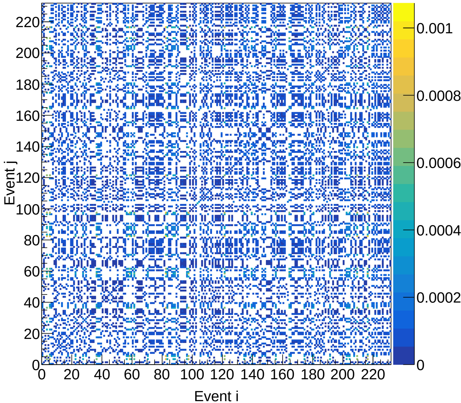
LH2 (total) Covariance | M: [4.8, 5.1) xF: [0.15, 0.20)
