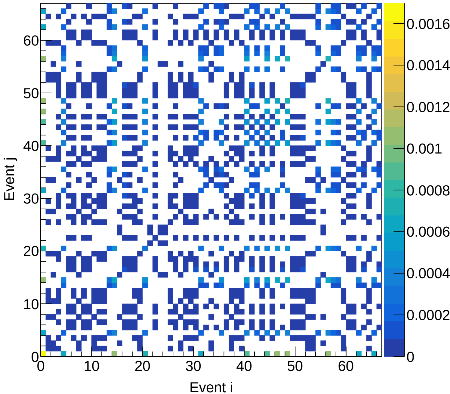
LH2 (total) Covariance | M: [6.0, 6.3) xF: [0.15, 0.20)
