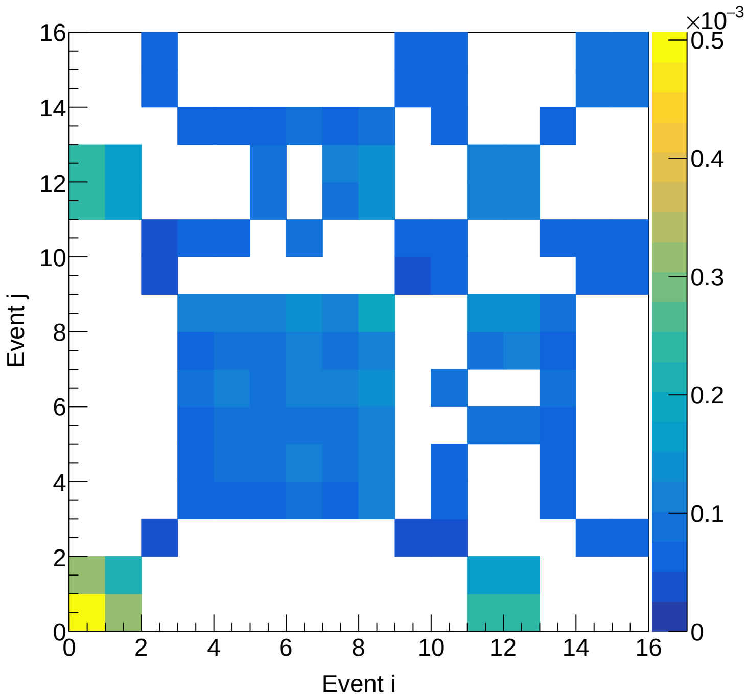
LH2 (total) Covariance | M: [6.6, 6.9] xF: [0.15, 0.20)
