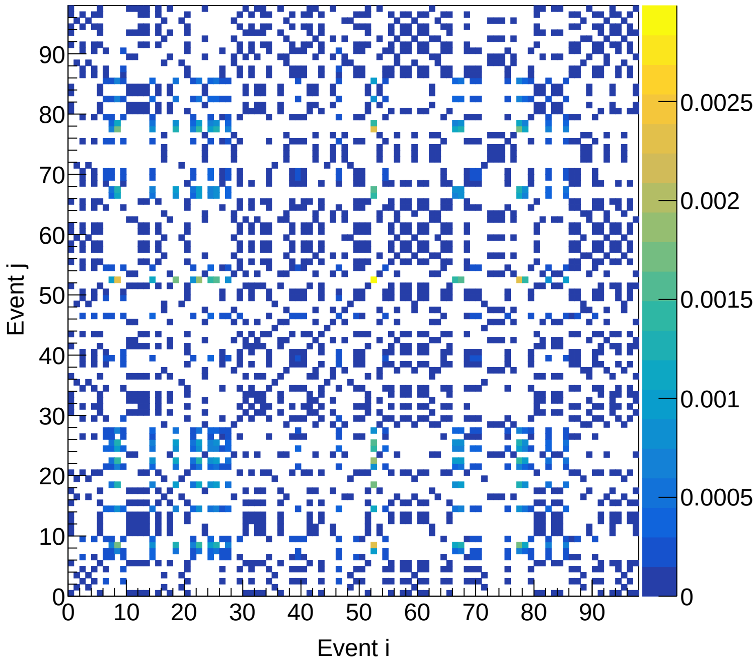
LH2 (total) Covariance | M: [3.9, 4.2) xF: [0.20, 0.25)
