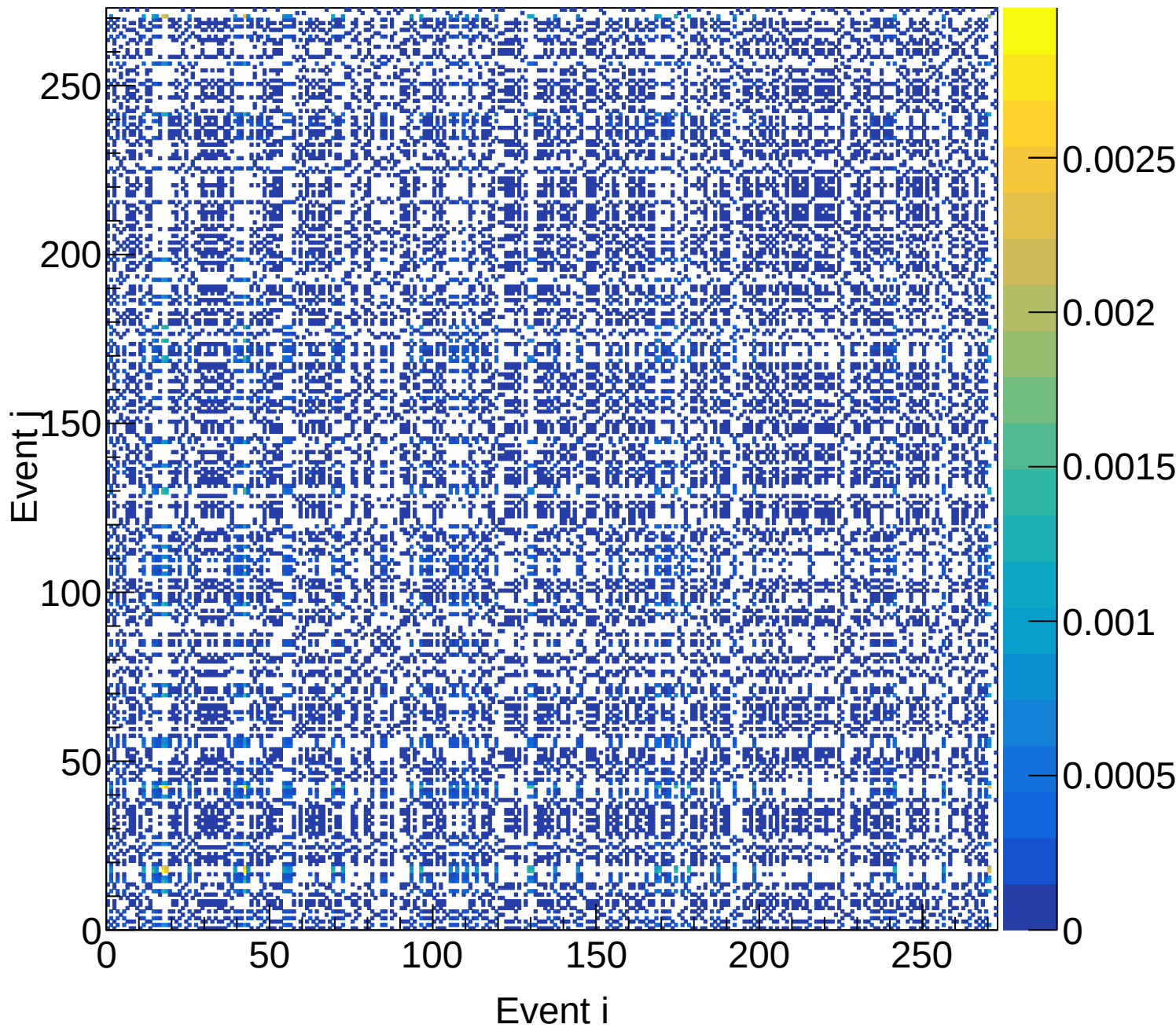
LH2 (total) Covariance | M: [4.8, 5.1) xF: [0.20, 0.25)
