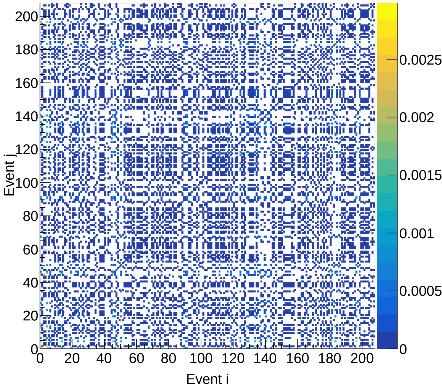
LH2 (total) Covariance | M: [5.1, 5.4) xF: [0.20, 0.25)
