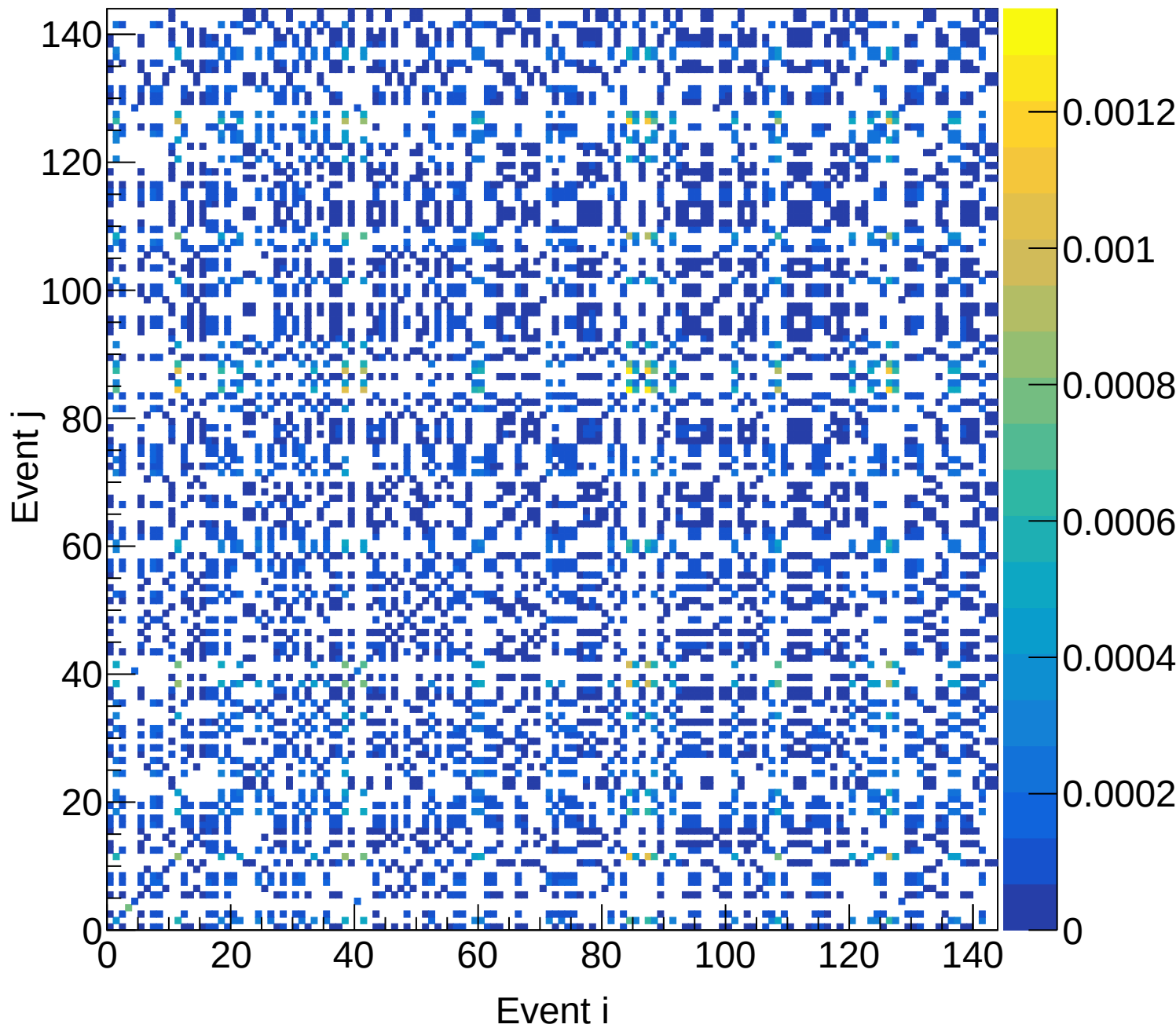
LH2 (total) Covariance | M: [5.4, 5.7) xF: [0.20, 0.25)
