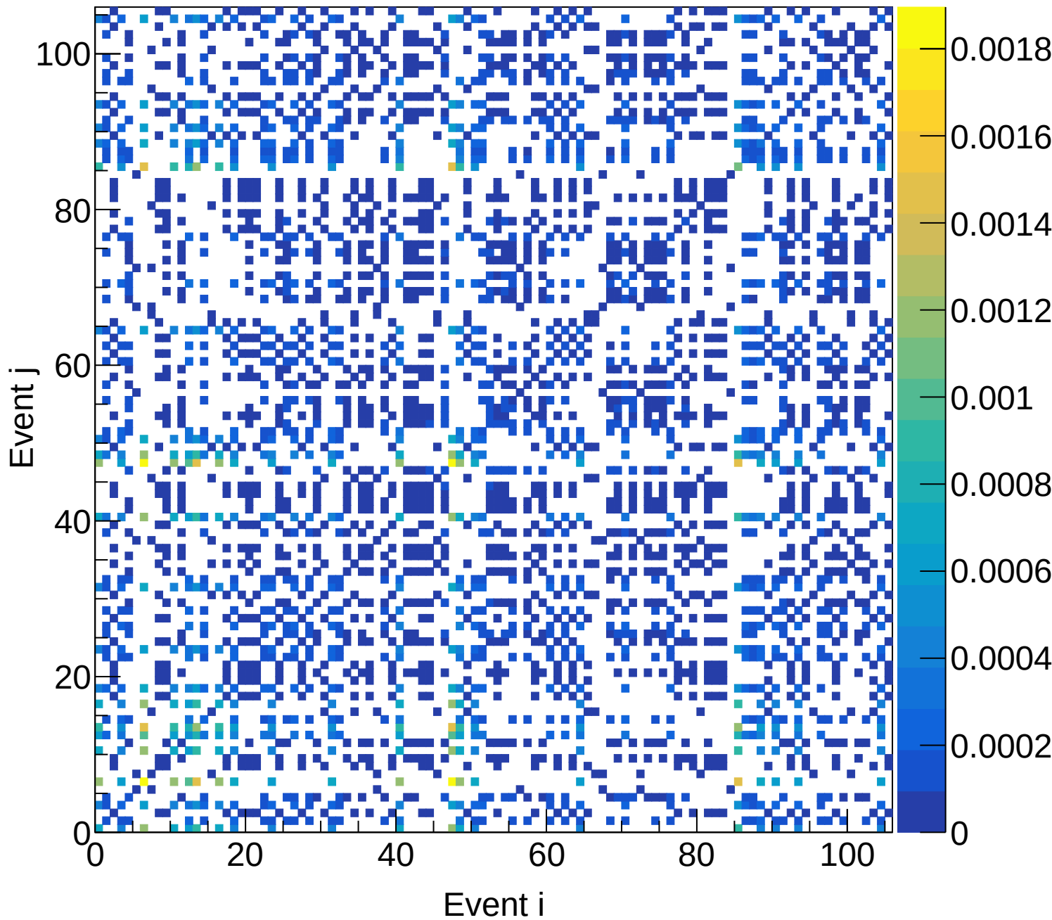
LH2 (total) Covariance | M: [5.7, 6.0] xF: [0.20, 0.25)
