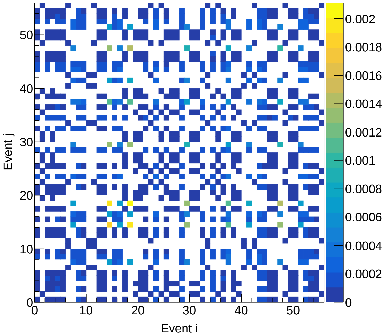
LH2 (total) Covariance | M: [6.0, 6.3) xF: [0.20, 0.25)
