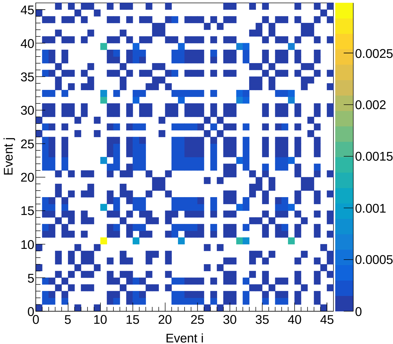
LH2 (total) Covariance | M: [6.3, 6.6) xF: [0.20, 0.25)
