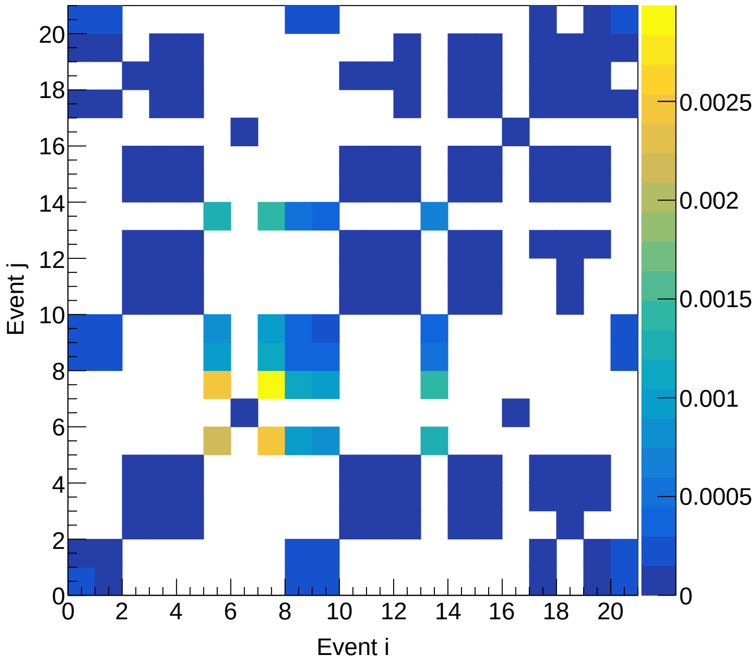
LH2 (total) Covariance | M: [6.6, 6.9] xF: [0.20, 0.25)
