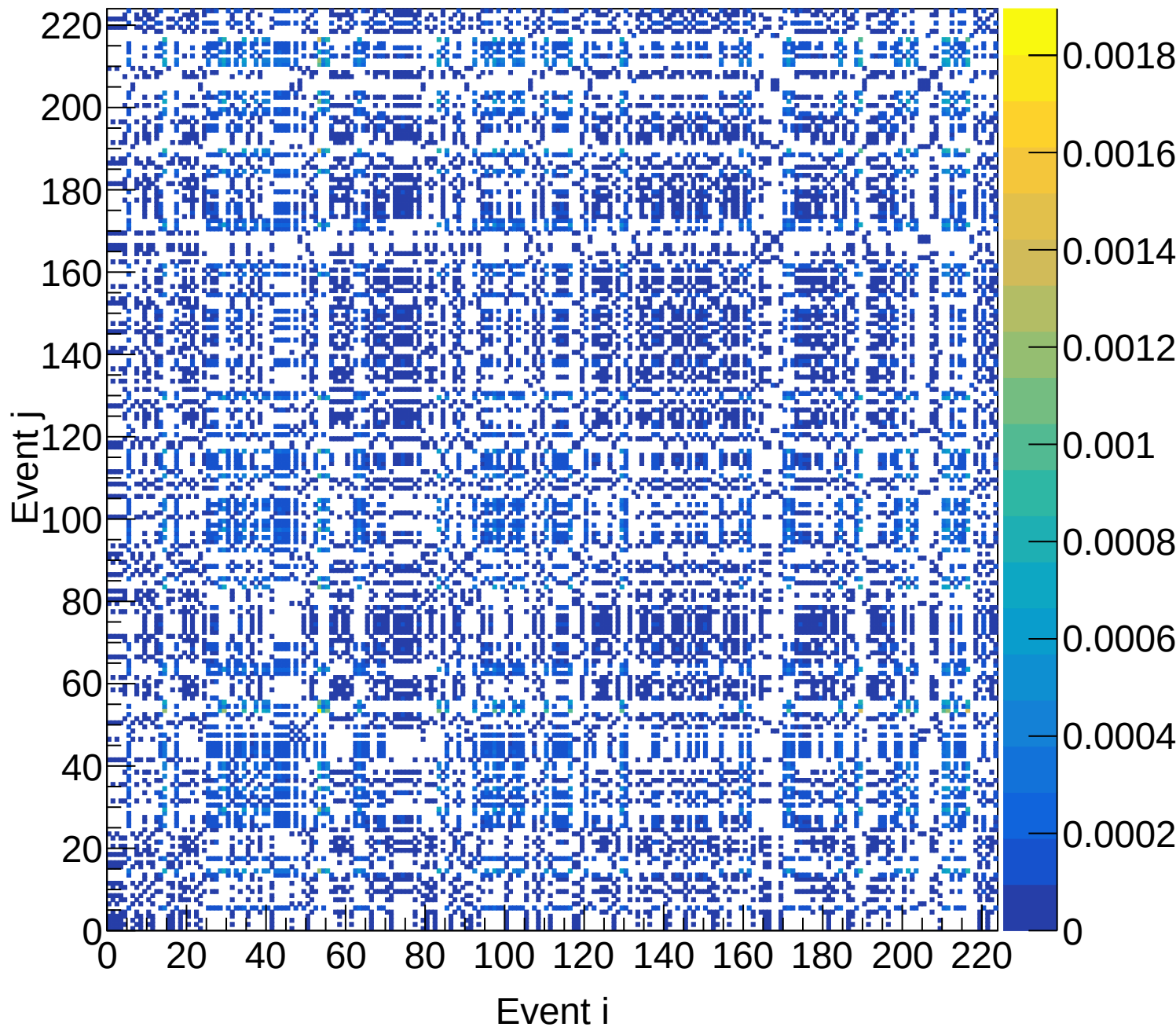
LH2 (total) Covariance | M: [3.9, 4.2) xF: [0.25, 0.30)
