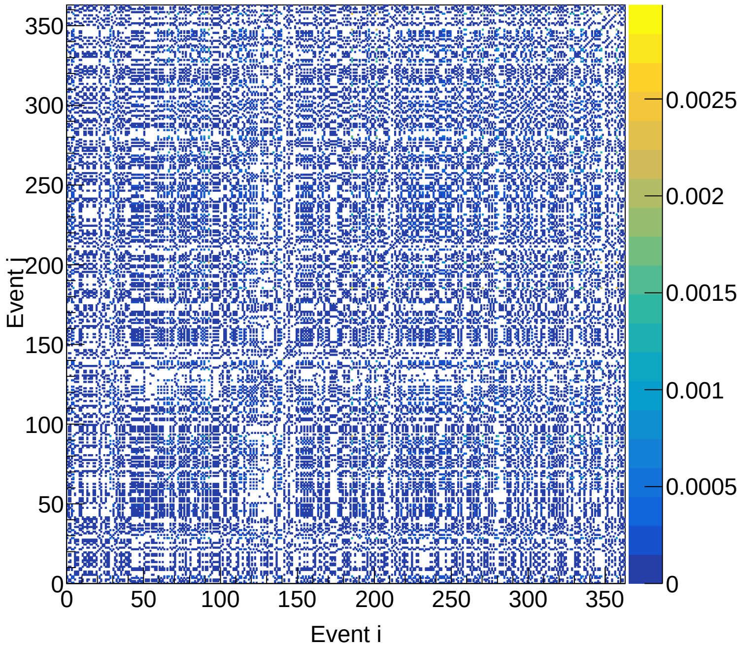
LH2 (total) Covariance | M: [4.2, 4.5) xF: [0.25, 0.30)
