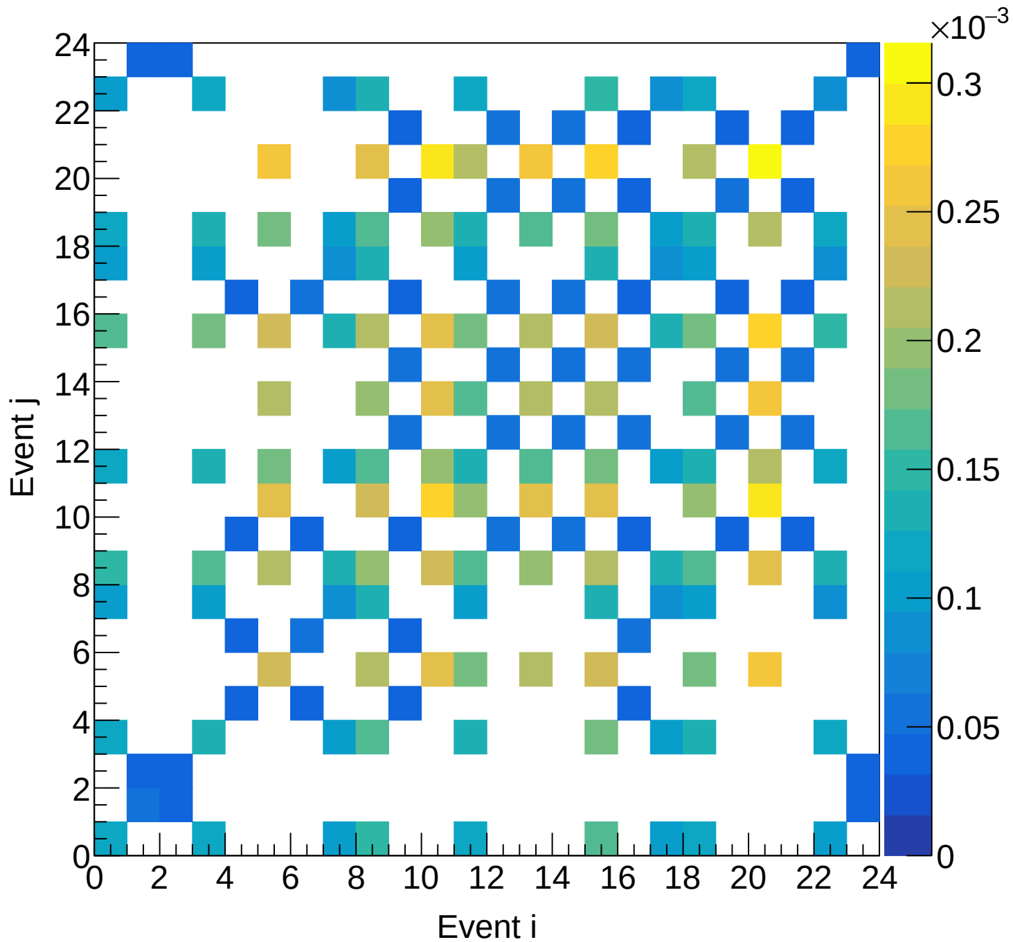
LH2 (total) Covariance | M: [6.9, 7.5) xF: [0.25, 0.30)
