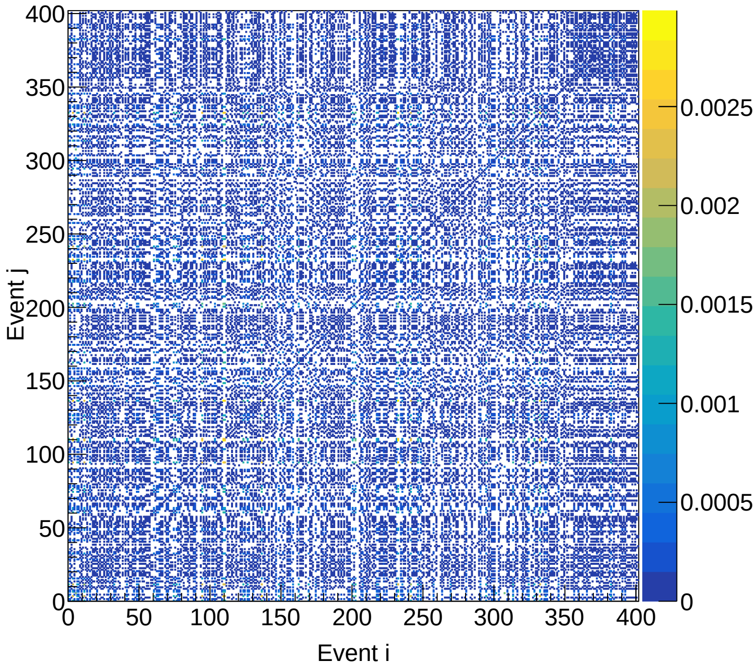
LH2 (total) Covariance | M: [4.5, 4.8) xF: [0.25, 0.30)
