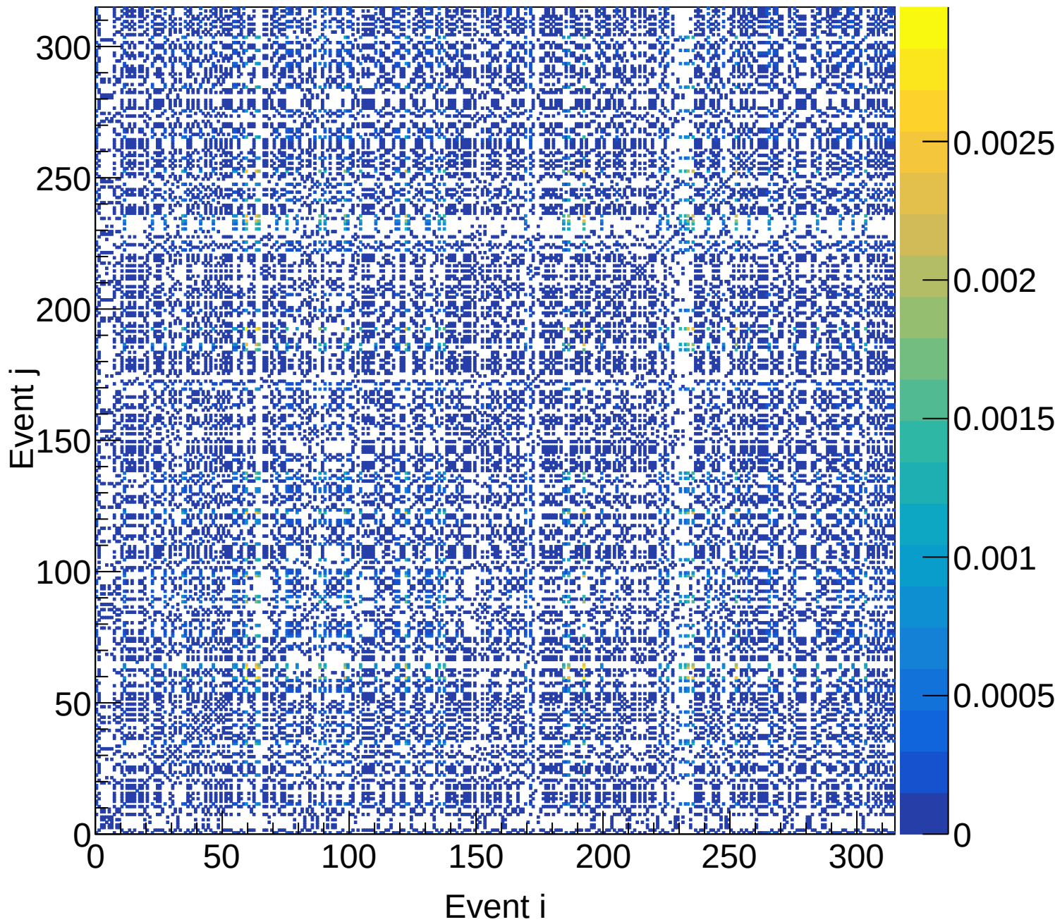
LH2 (total) Covariance | M: [4.8, 5.1) xF: [0.25, 0.30)
