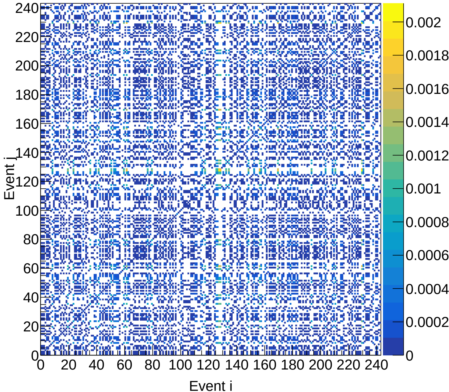
LH2 (total) Covariance | M: [5.1, 5.4) xF: [0.25, 0.30)
