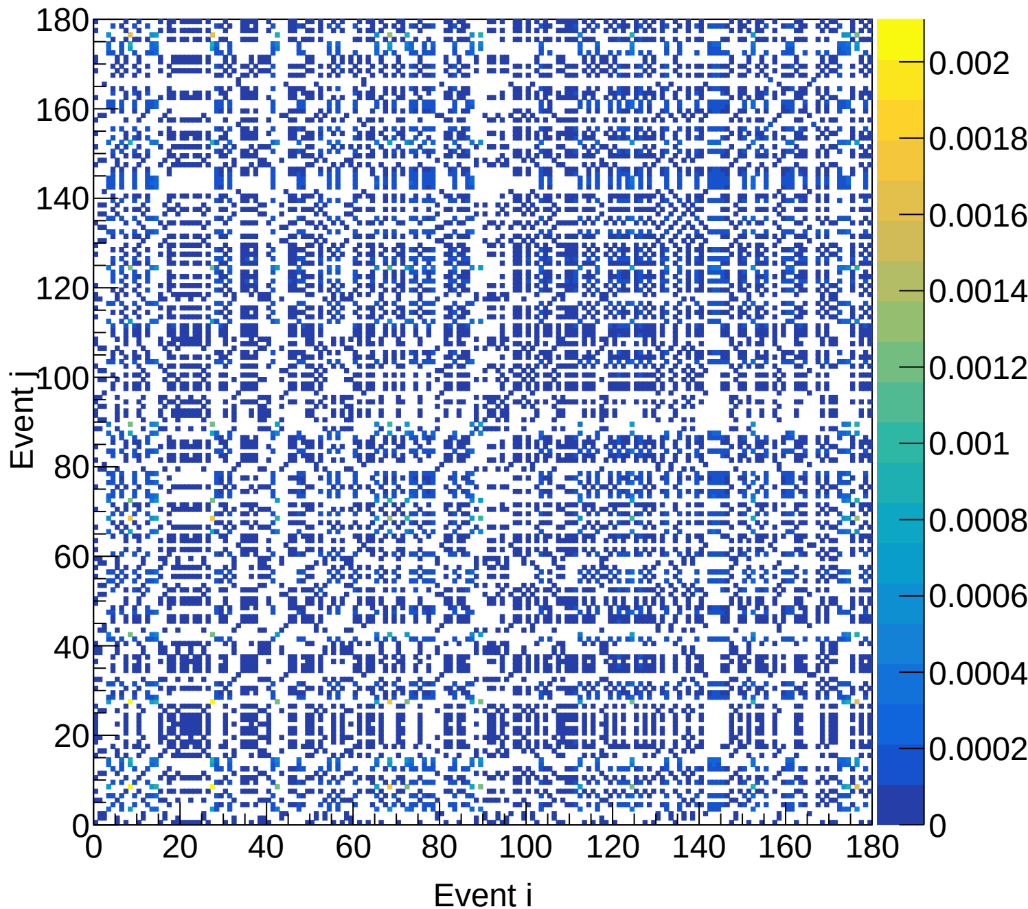
LH2 (total) Covariance | M: [5.4, 5.7) xF: [0.25, 0.30)
