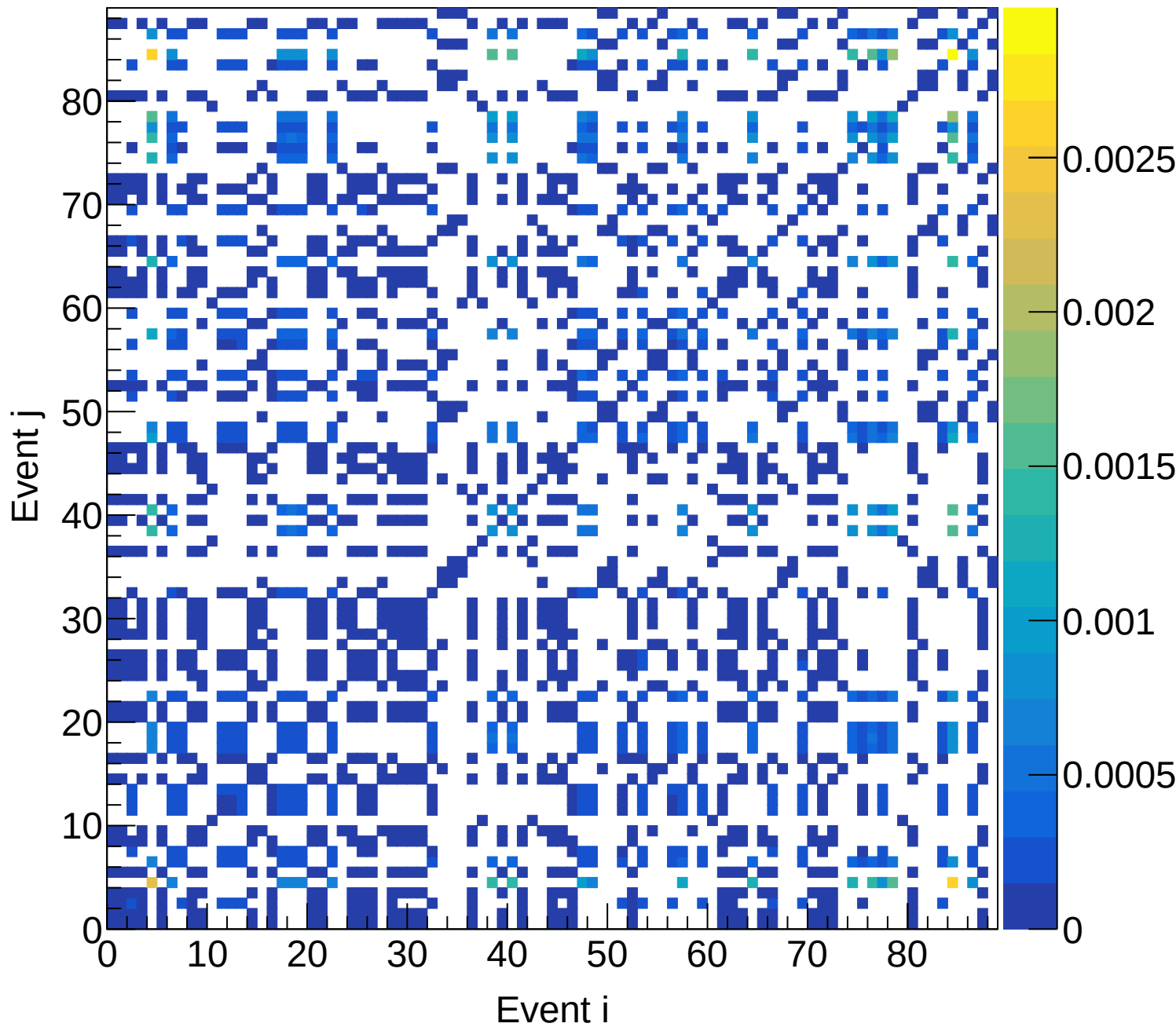
LH2 (total) Covariance | M: [5.7, 6.0] xF: [0.25, 0.30)
