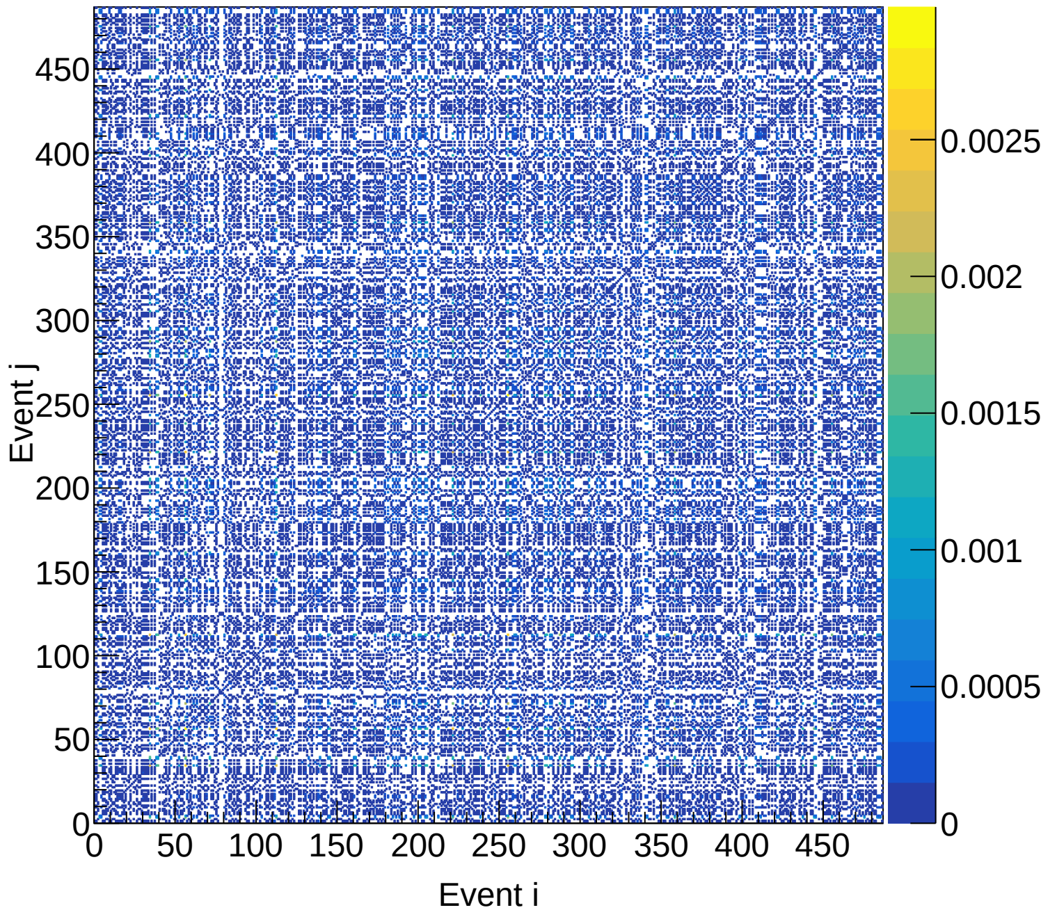
LH2 (total) Covariance | M: [3.9, 4.2) xF: [0.30, 0.35)
