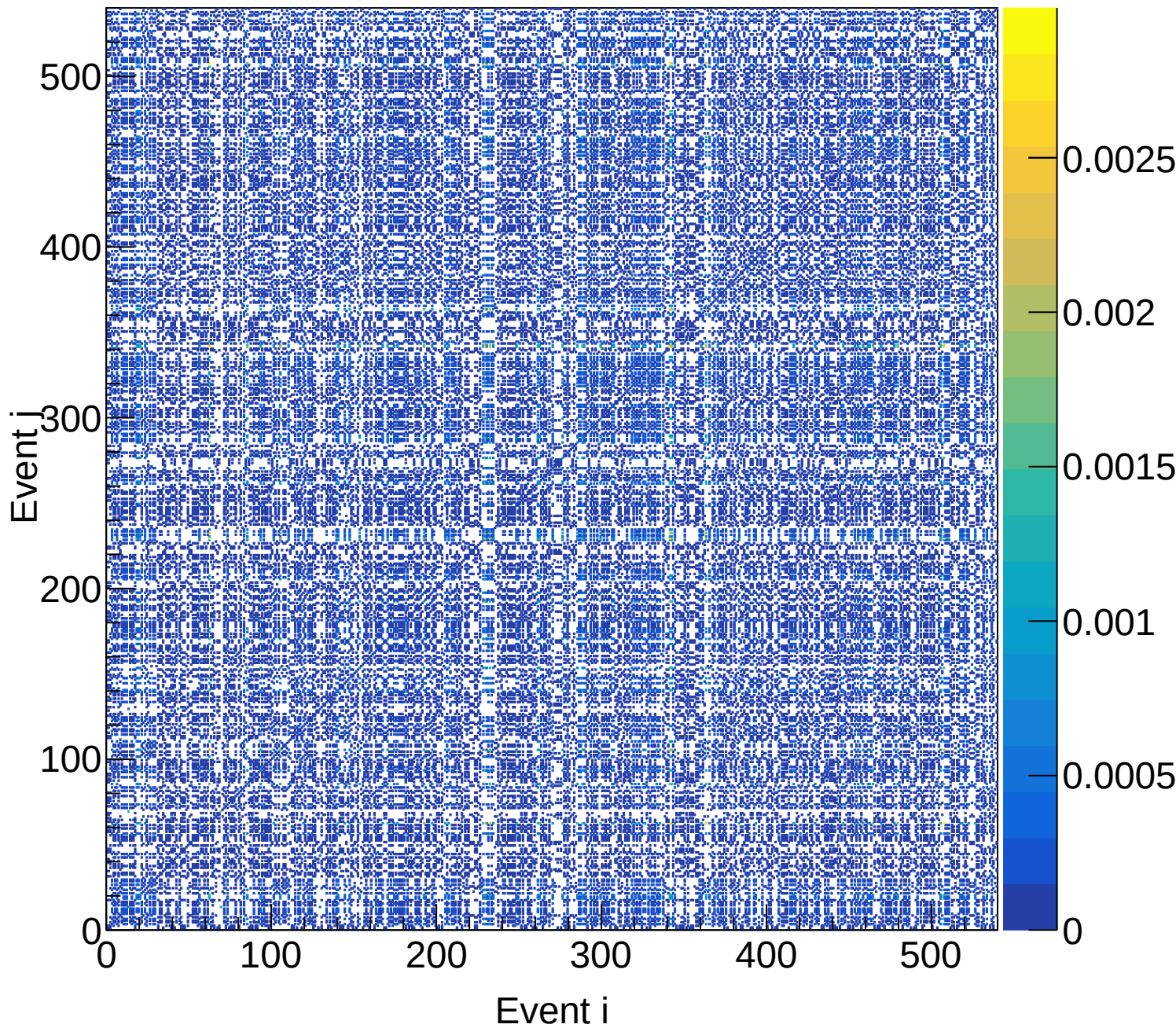
LH2 (total) Covariance | M: [4.2, 4.5) xF: [0.30, 0.35)
