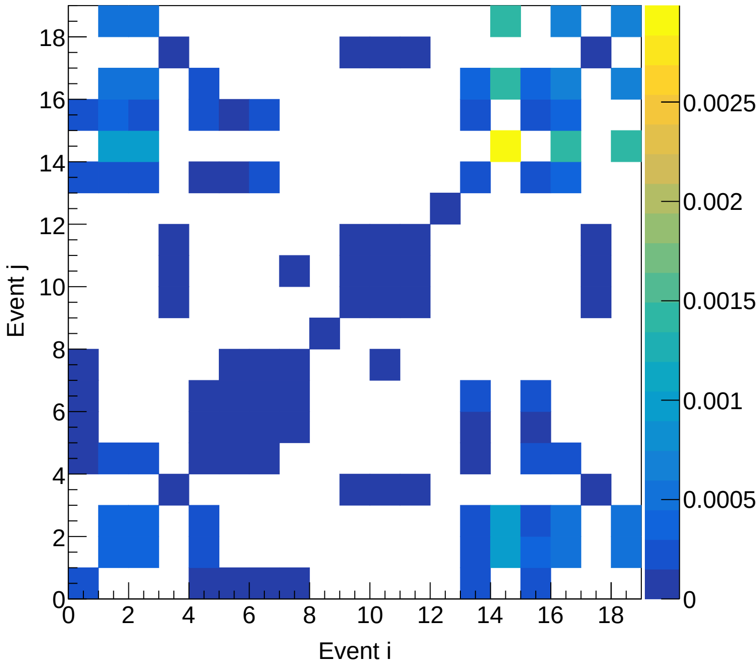
LH2 (total) Covariance | M: [6.9, 7.5) xF: [0.30, 0.35)
