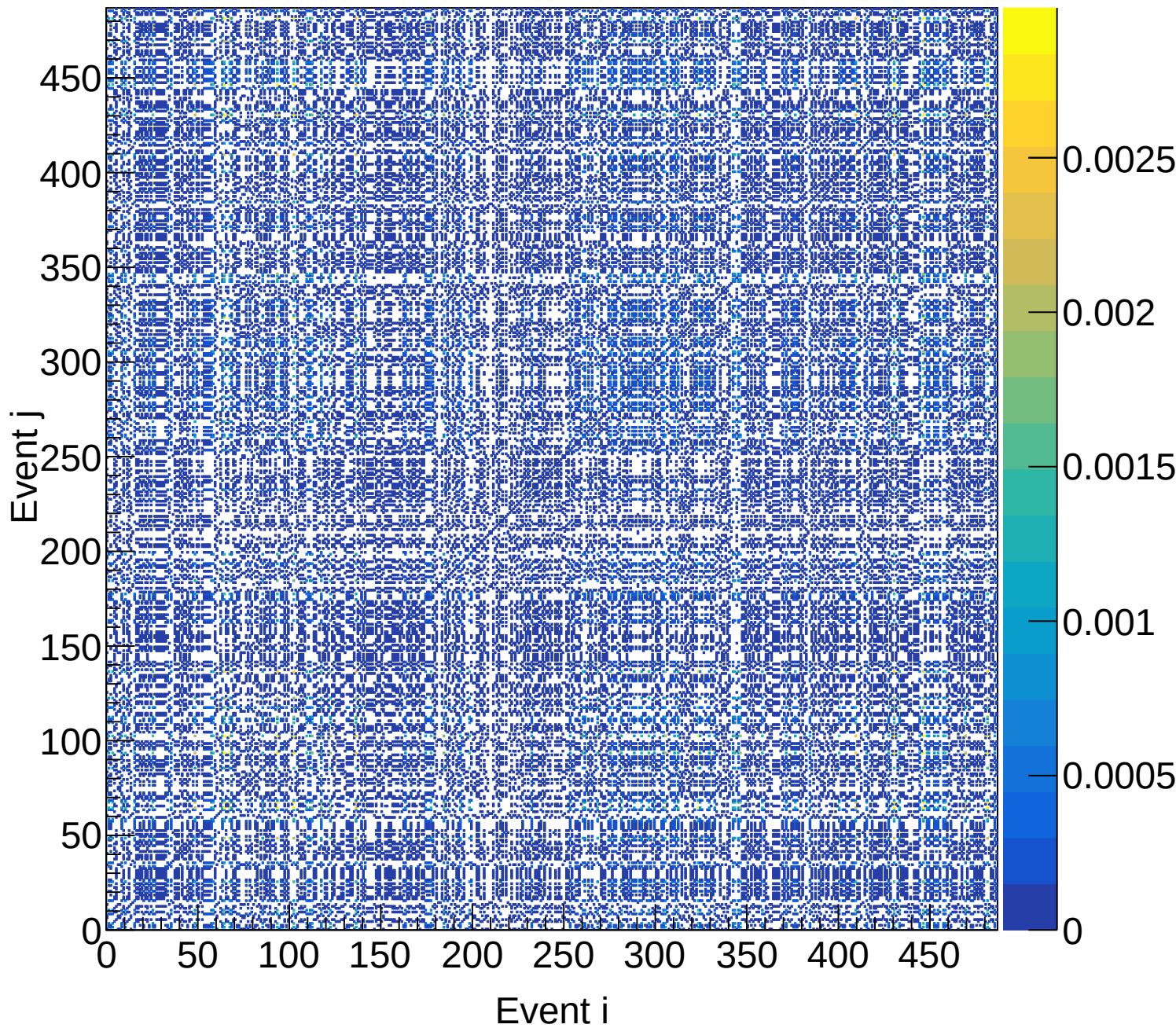
LH2 (total) Covariance | M: [4.5, 4.8) xF: [0.30, 0.35)
