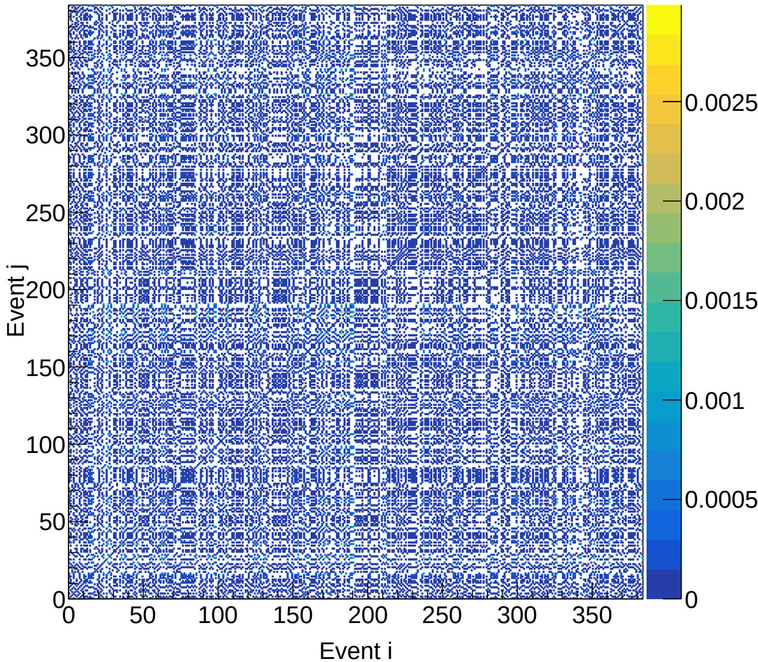
LH2 (total) Covariance | M: [4.8, 5.1) xF: [0.30, 0.35)
