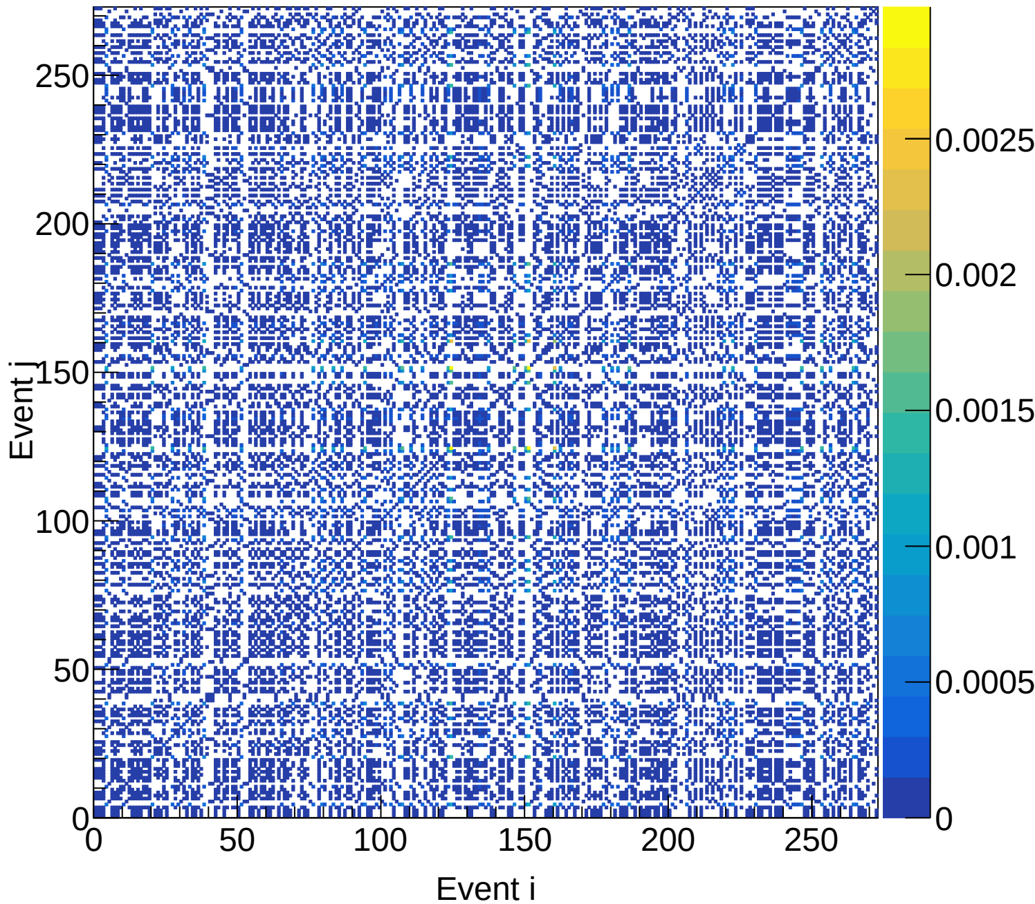
LH2 (total) Covariance | M: [5.1, 5.4) xF: [0.30, 0.35)
