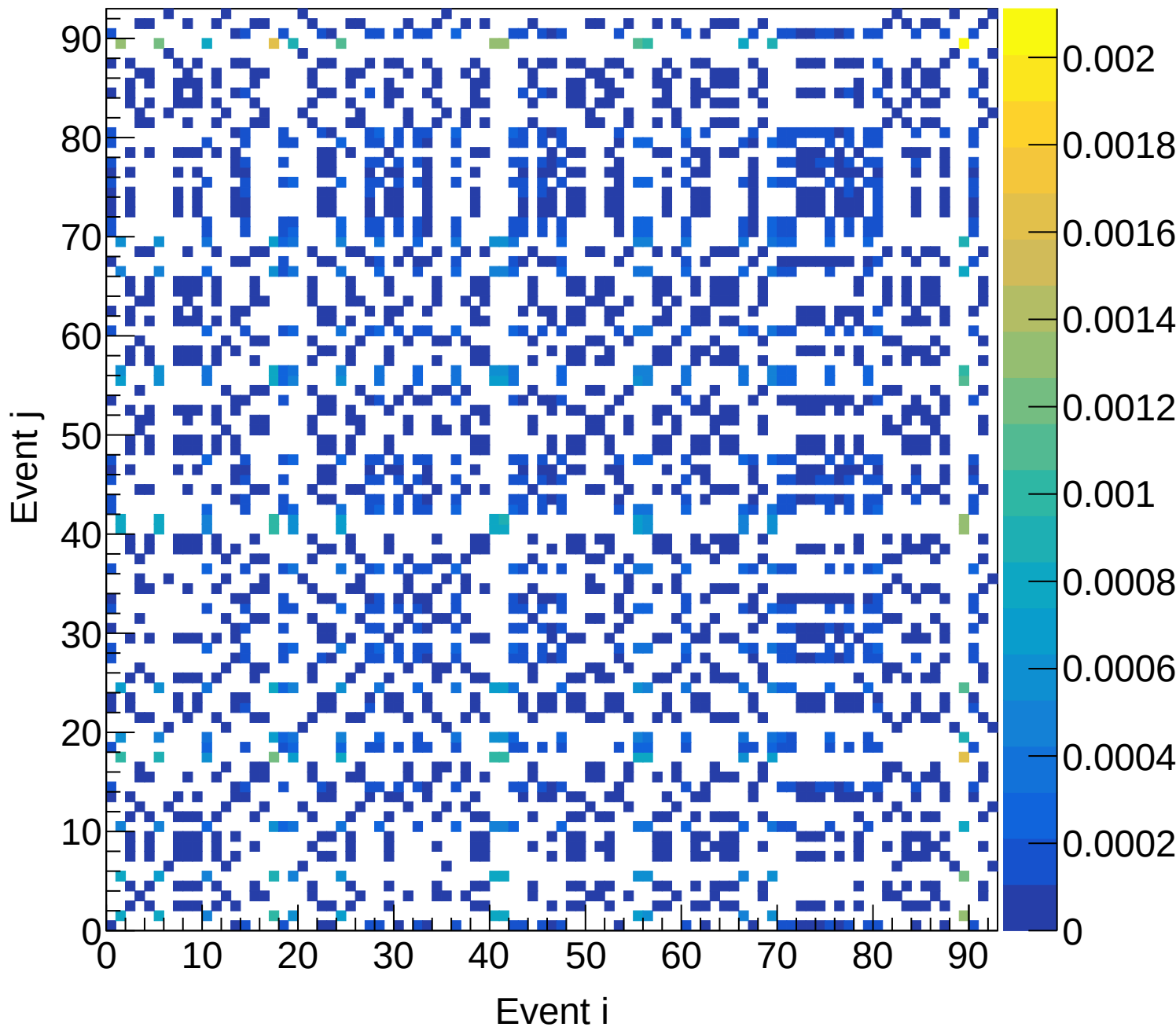
LH2 (total) Covariance | M: [5.7, 6.0) xF: [0.30, 0.35)
