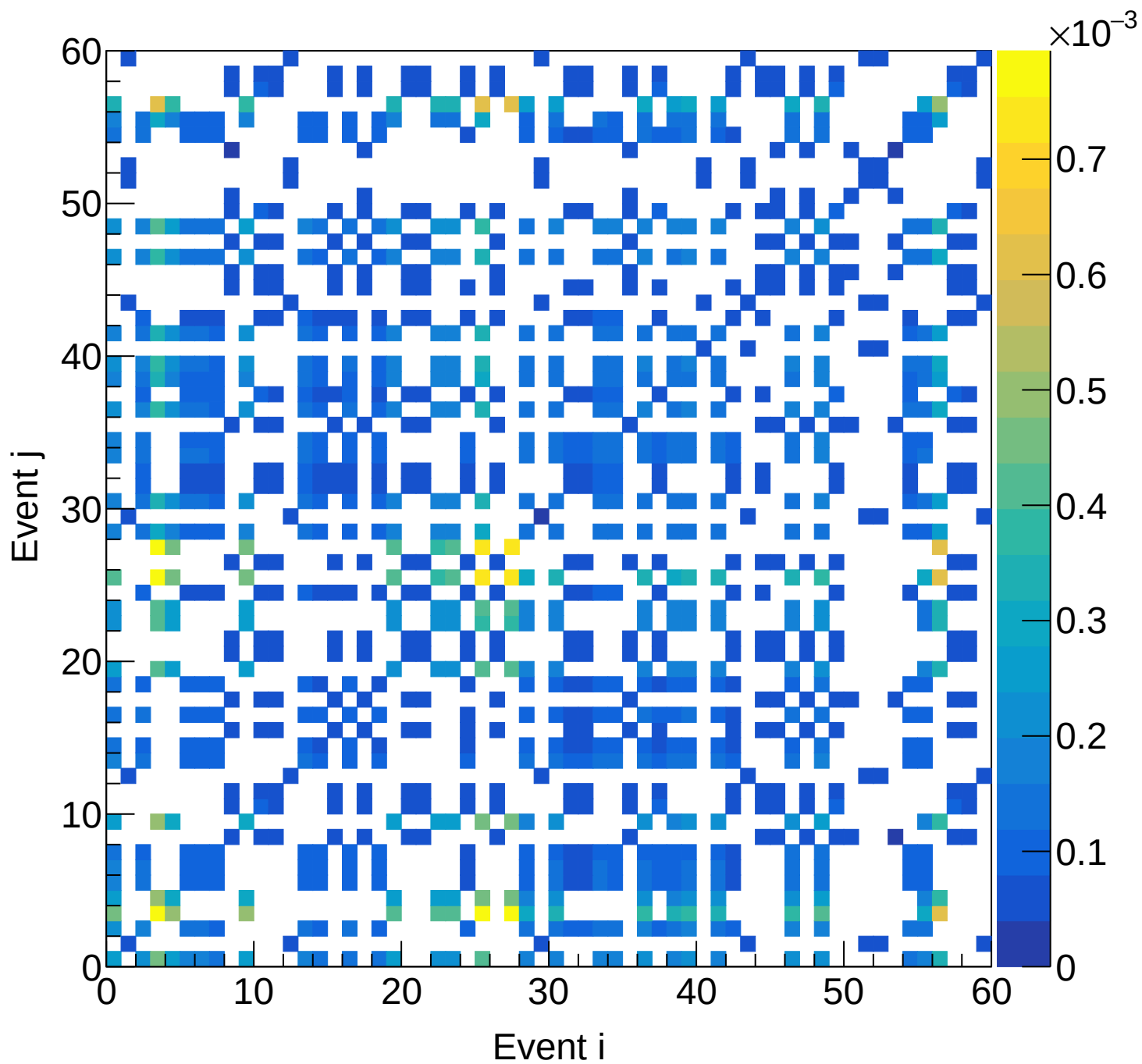
LH2 (total) Covariance | M: [6.0, 6.3) xF: [0.30, 0.35)
