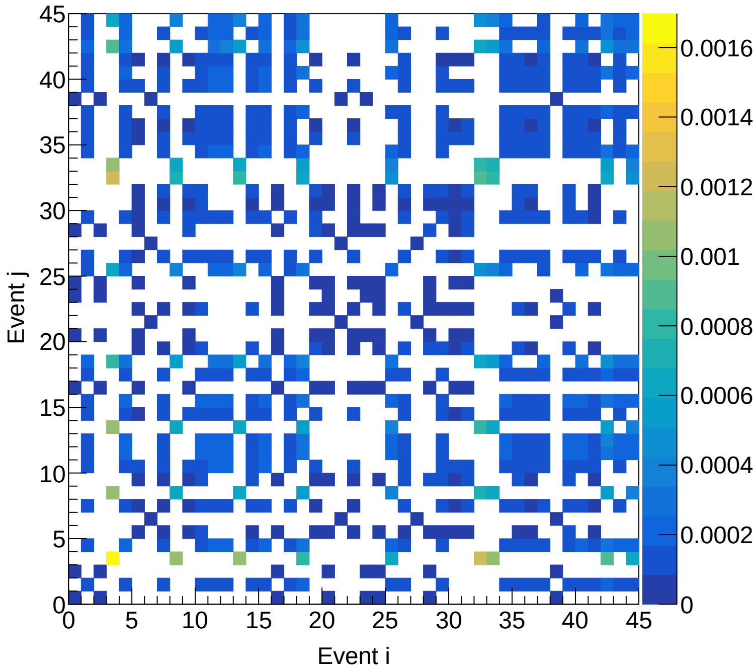
LH2 (total) Covariance | M: [6.3, 6.6) xF: [0.30, 0.35)
