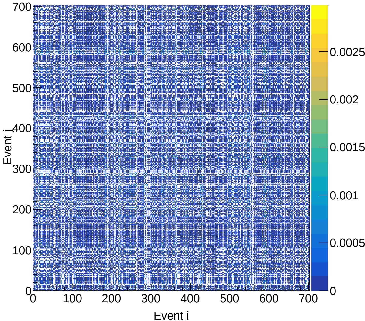
LH2 (total) Covariance | M: [3.9, 4.2) xF: [0.35, 0.40)
