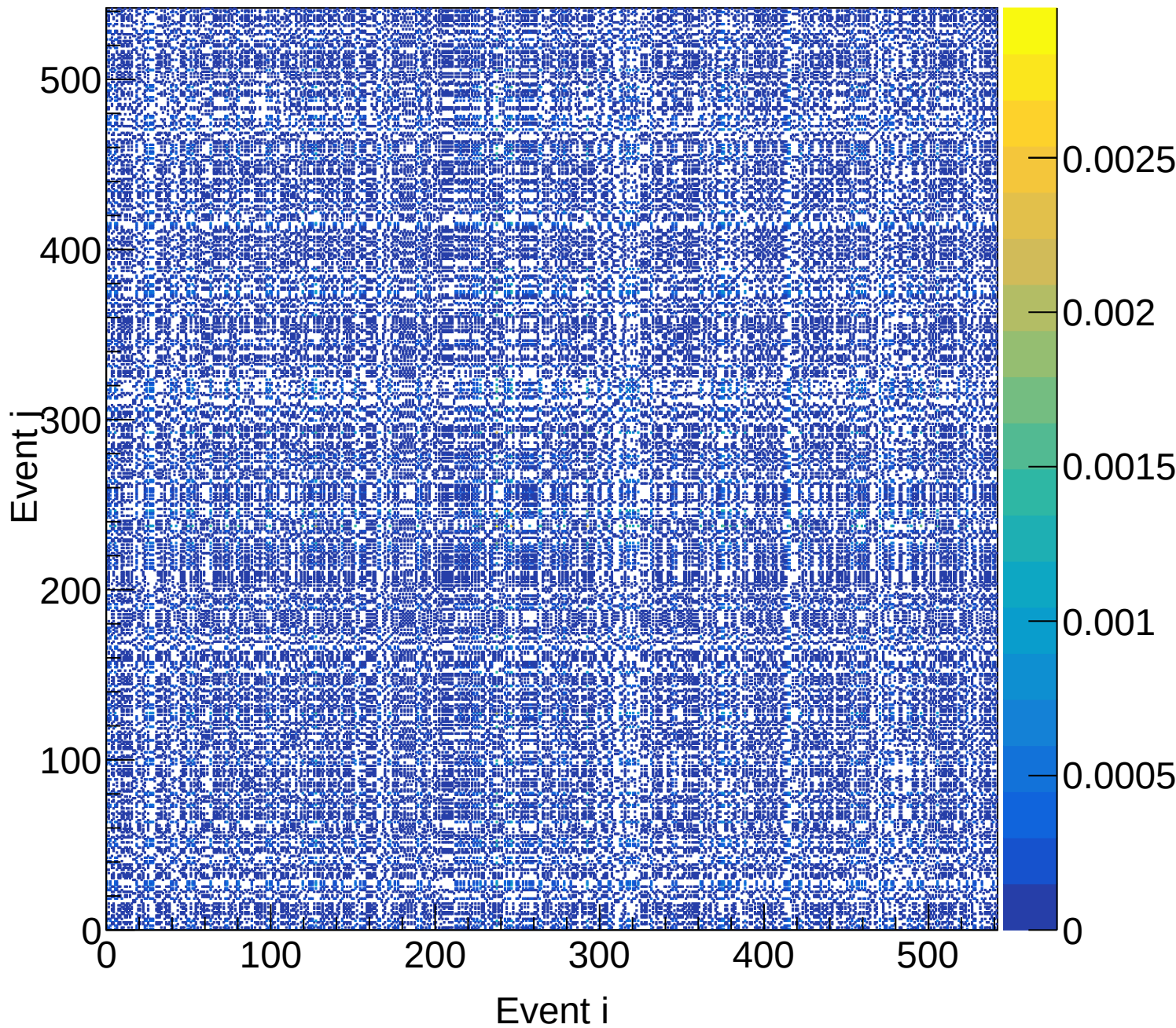
LH2 (total) Covariance | M: [4.5, 4.8) xF: [0.35, 0.40)
