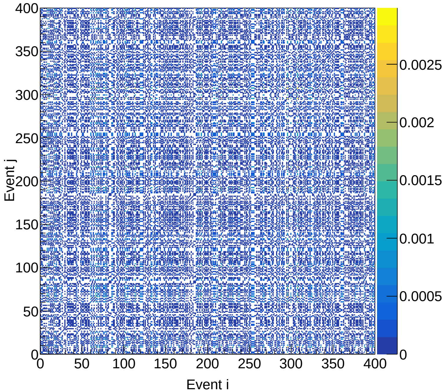
LH2 (total) Covariance | M: [4.8, 5.1) xF: [0.35, 0.40)
