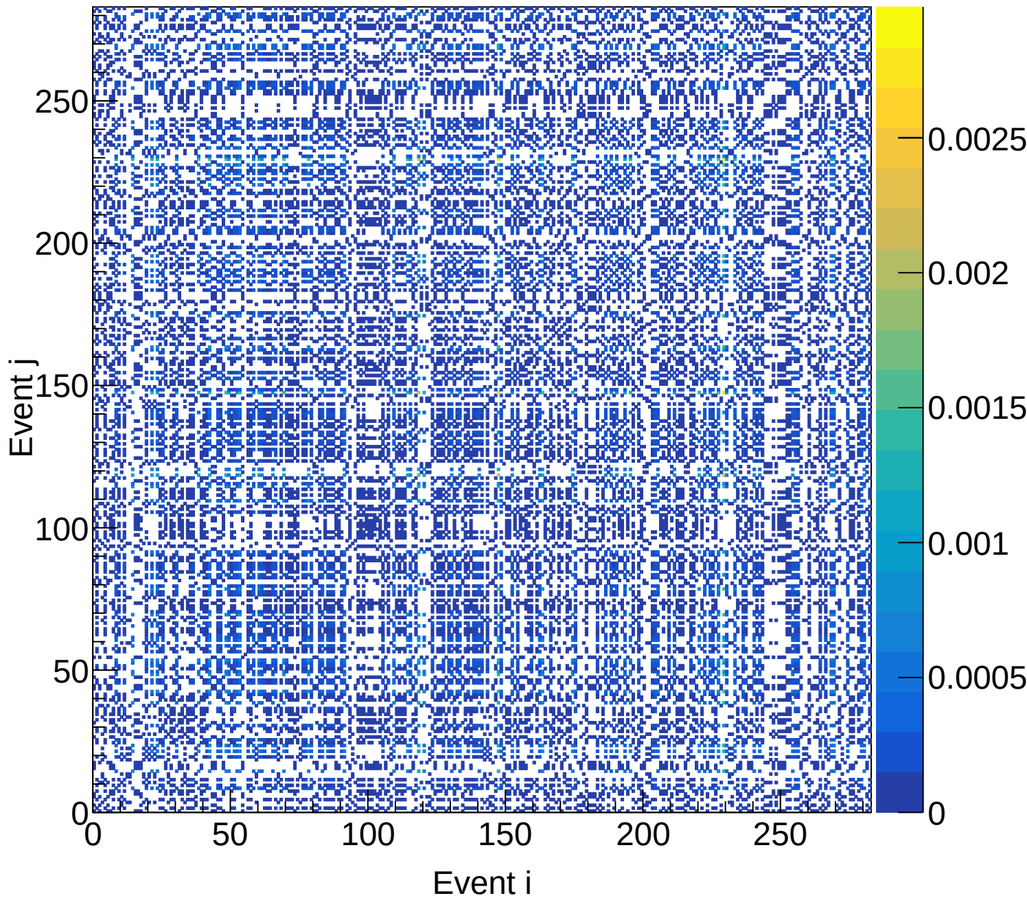
LH2 (total) Covariance | M: [5.1, 5.4) xF: [0.35, 0.40)
