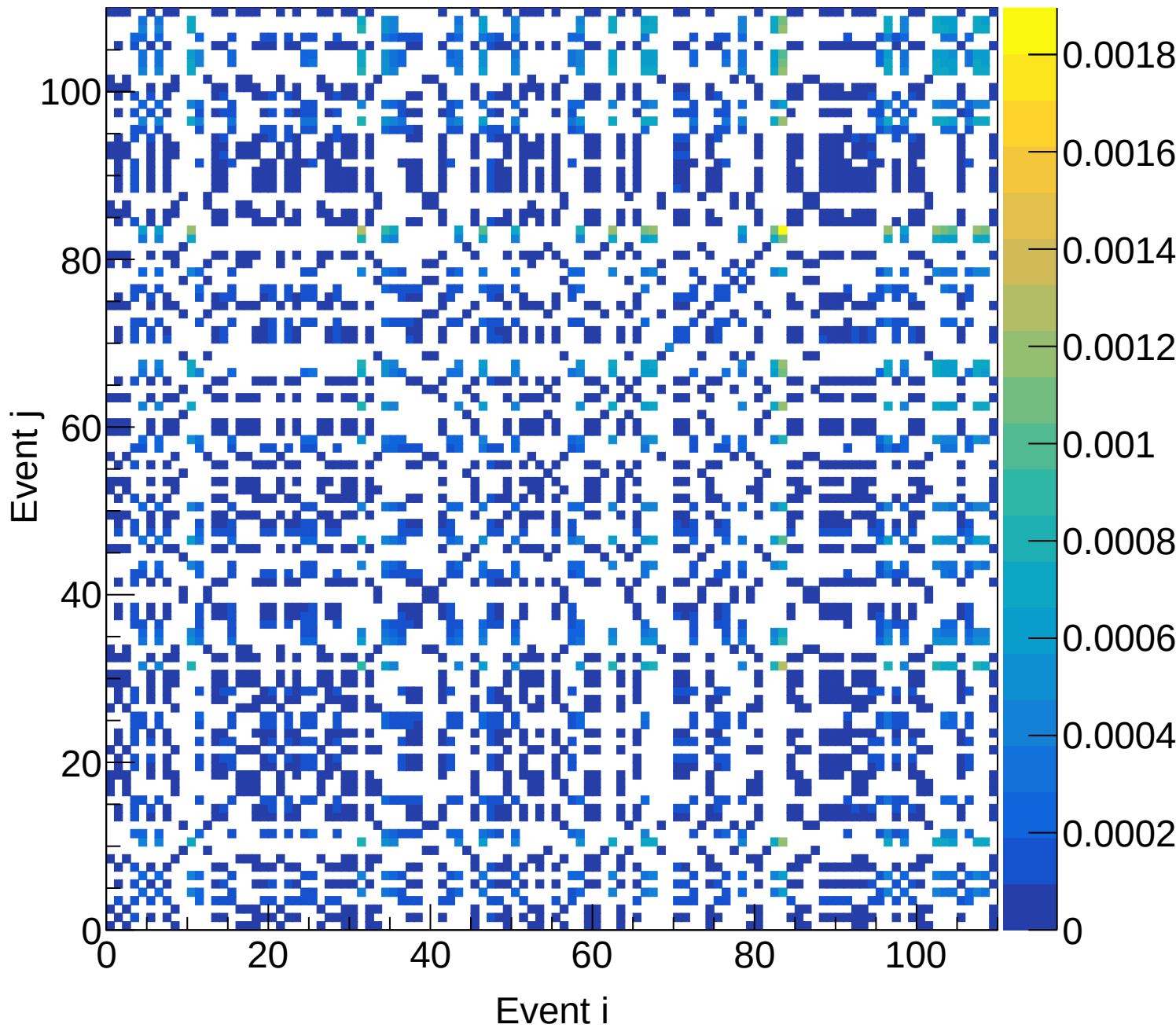
LH2 (total) Covariance | M: [5.7, 6.0] xF: [0.35, 0.40]
