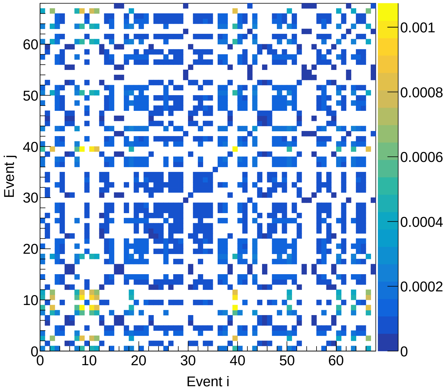
LH2 (total) Covariance | M: [6.0, 6.3] xF: [0.35, 0.40]
