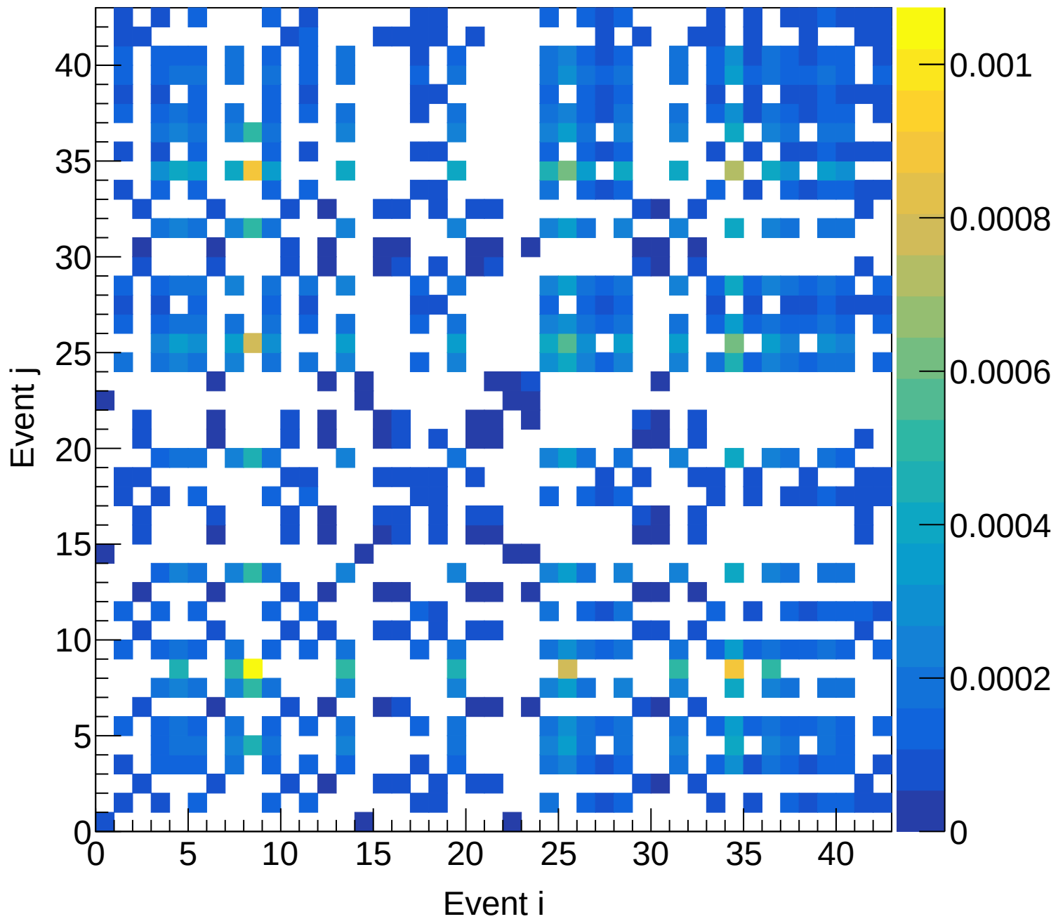
LH2 (total) Covariance | M: [6.3, 6.6) xF: [0.35, 0.40)
