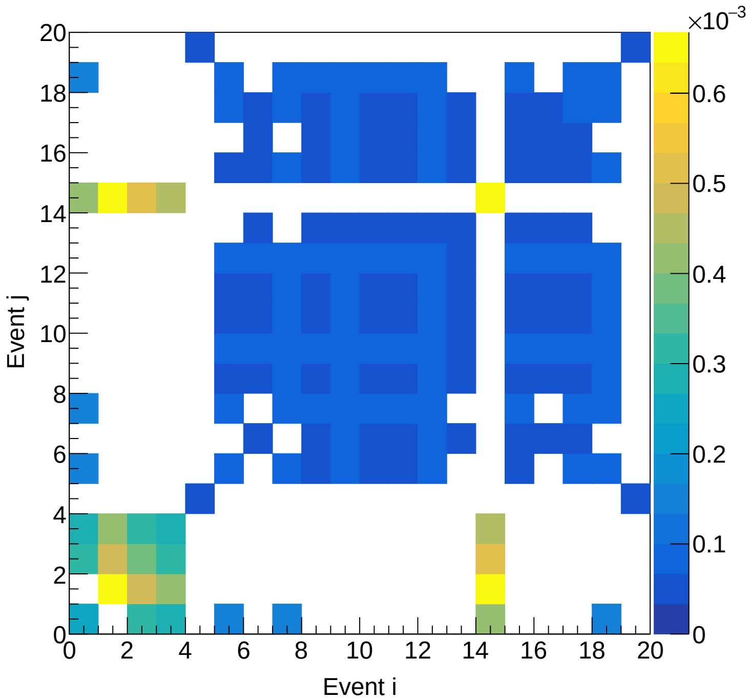
LH2 (total) Covariance | M: [6.6, 6.9) xF: [0.35, 0.40)
